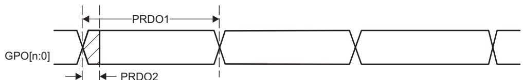
Figure 5-109. PRU-ICSS PRU Direct Output Timing
