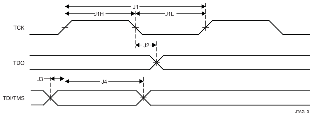
Figure 5-129. JTAG Timing
