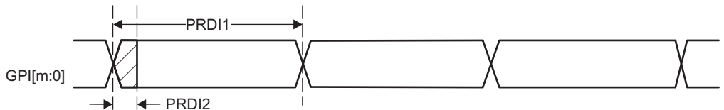
Figure 5-108. PRU-ICSS PRU Direct Input Timing
