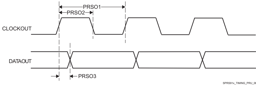
Figure 5-113. PRU-ICSS PRU Shift Out Timing
