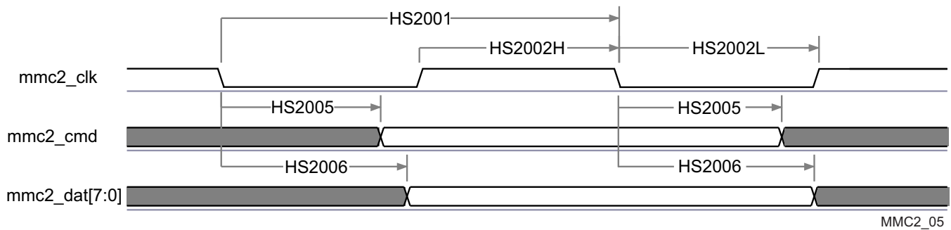
Figure 5-95. eMMC in - HS200 SDR - Transmitter Mode
