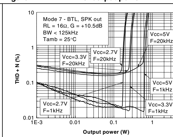
Figure 21. THD+N vs. output power
