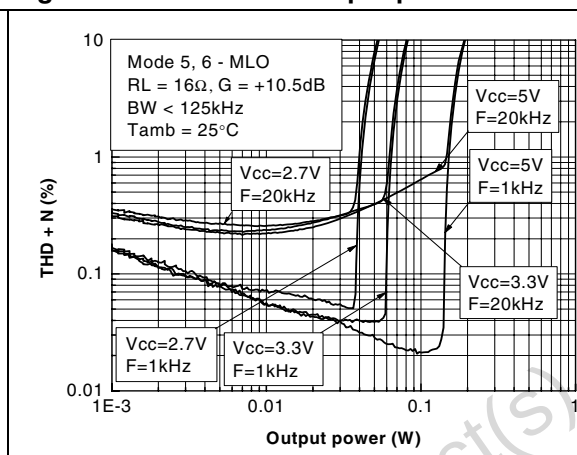
Figure 17. THD+N vs. output power
