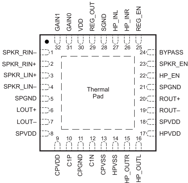
TPA6045A4CRHB (TOP VIEW)
