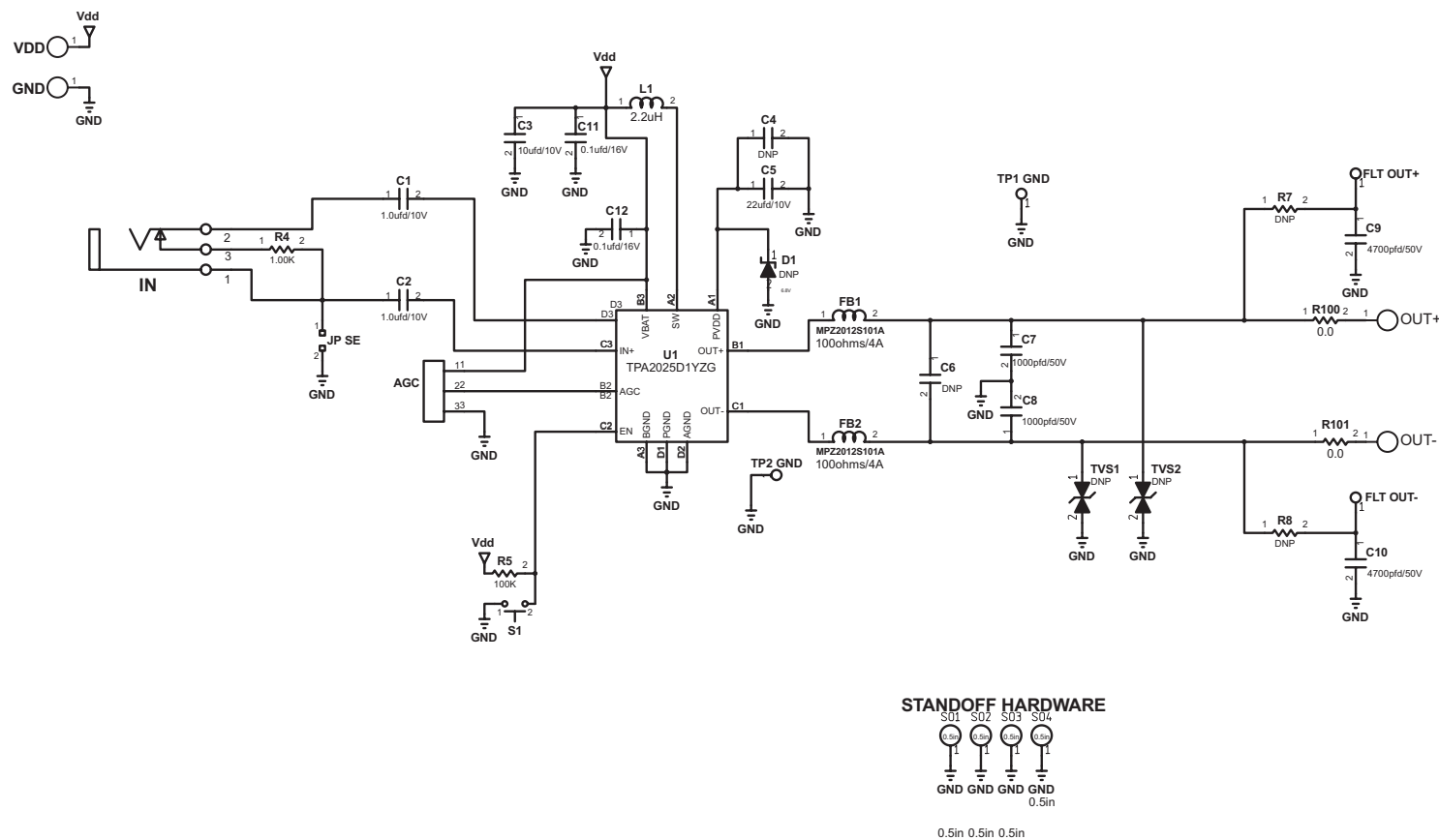
Figure 1. TPA2025D1EVM Schematic
