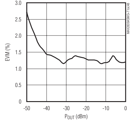
EVM vs. Tx OUTPUT POWER (64 QAM FUSC, 10MHz CHANNEL BANDWIDTH)
