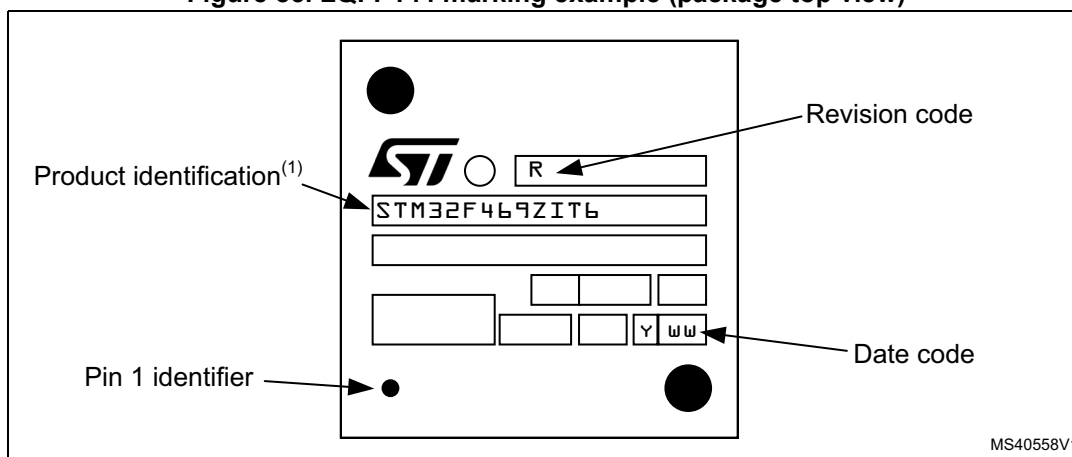
Figure 85. LQFP144 marking example (package top view)
