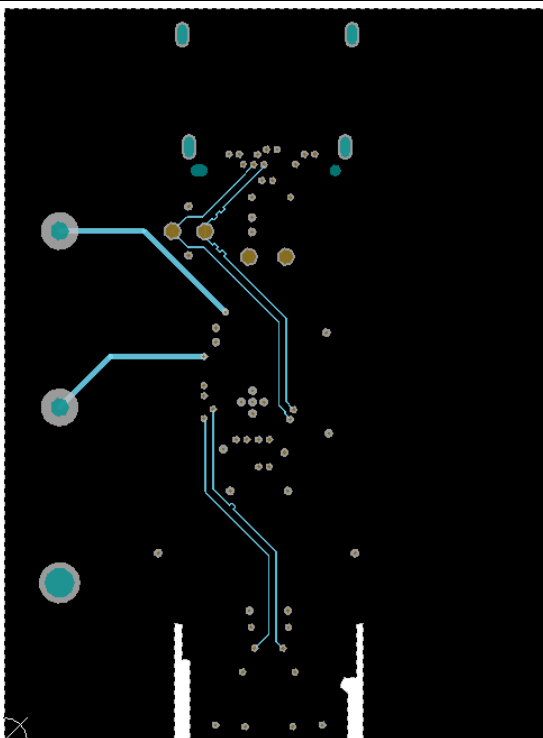
Figure 6. Midlayer 1
