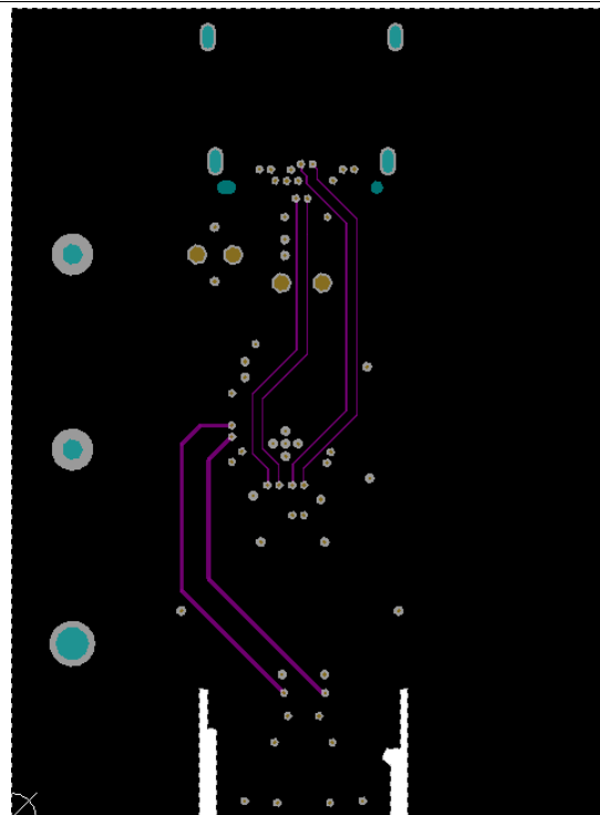
Figure 9. Midlayer 2
