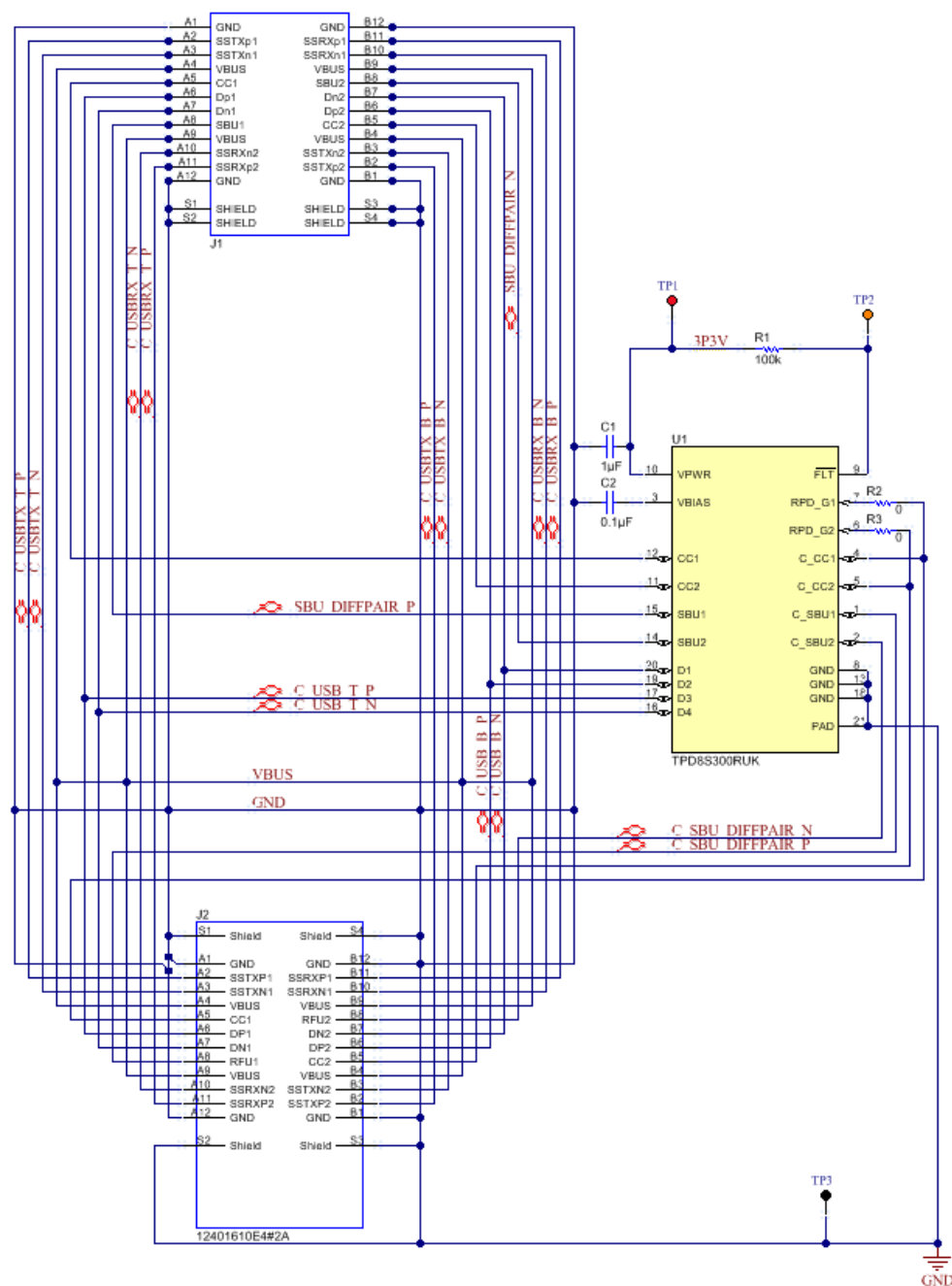
Figure 3. TPD8S300EVM Schematic
