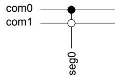
Figure 15.12. LCD 1/2 Bias and Duplex Multiplexing - LCD_SEG0 Connection
