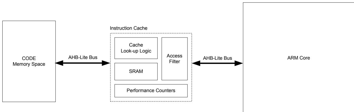
Figure 6.1. Instruction Cache
