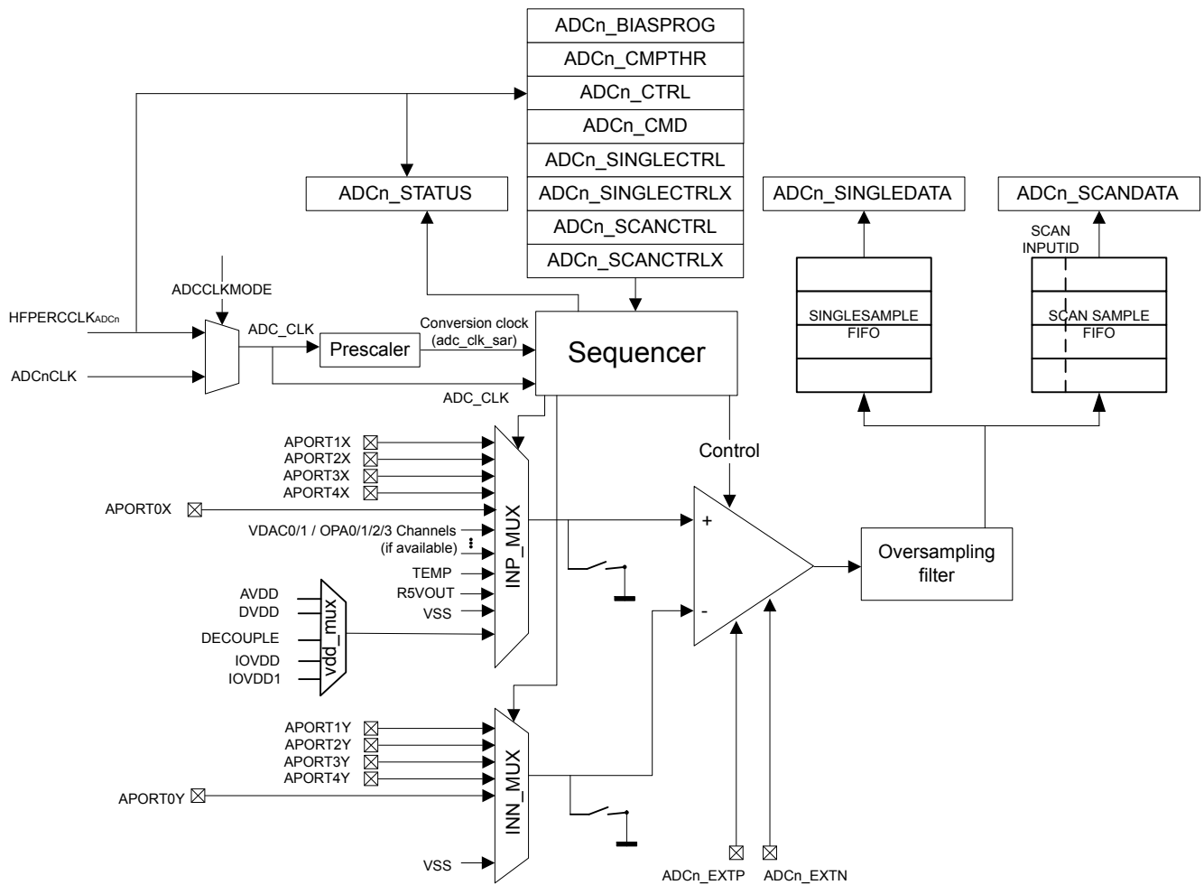
Figure 27.1. ADC Overview
