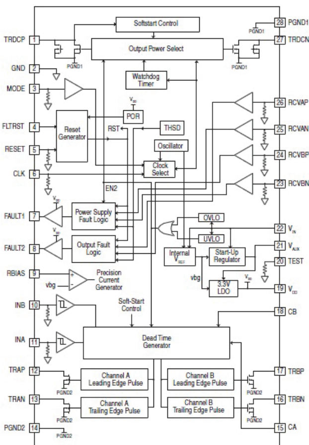
Figure 2: IX6610 Functional Block Diagram
