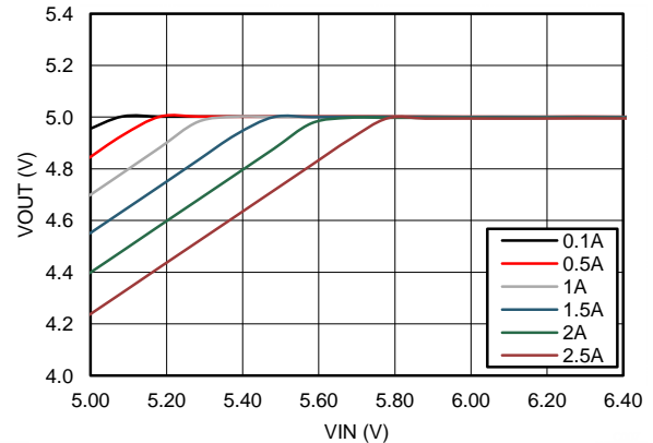
Figure 70. Dropout Curve
