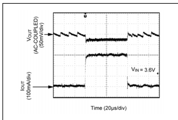
FIGURE 2-26: Load Transient (0 mA to 400 mA).
