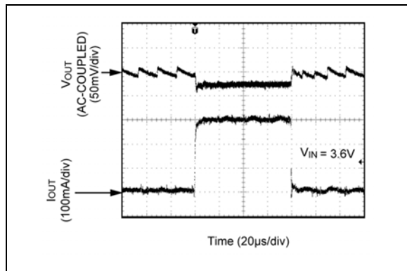
FIGURE 2-25: Load Transient 0 mA to 300 mA.
