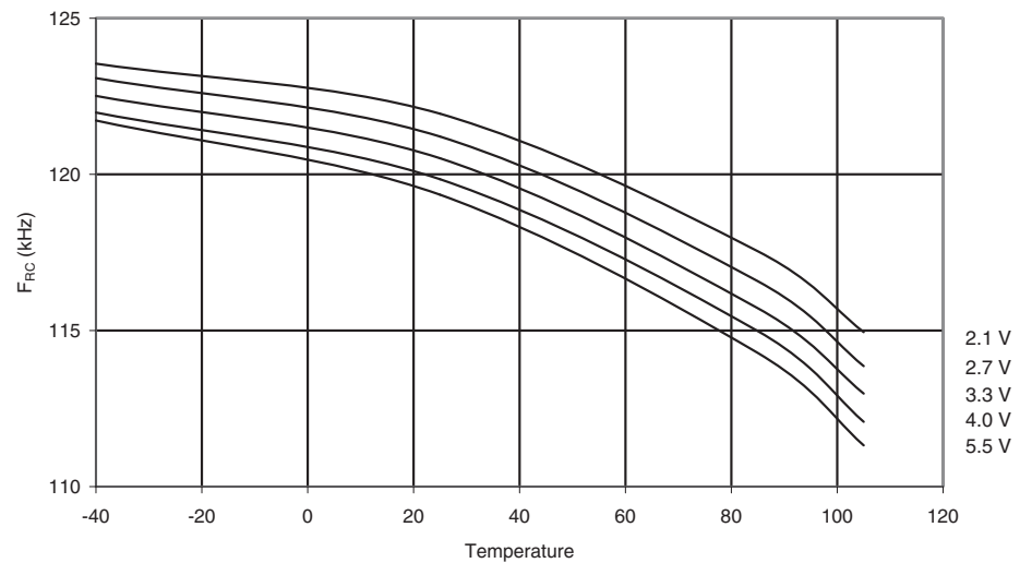
Figure 2-69. ATmega324P: Watchdog Oscillator Frequency vs. Temperature
