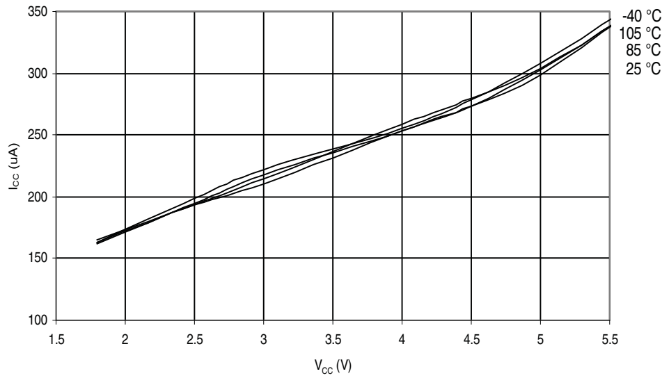
Figure 2-33. ATmega164P: ADC Current vs. V_{CC} (AREF = AV_{CC} )
