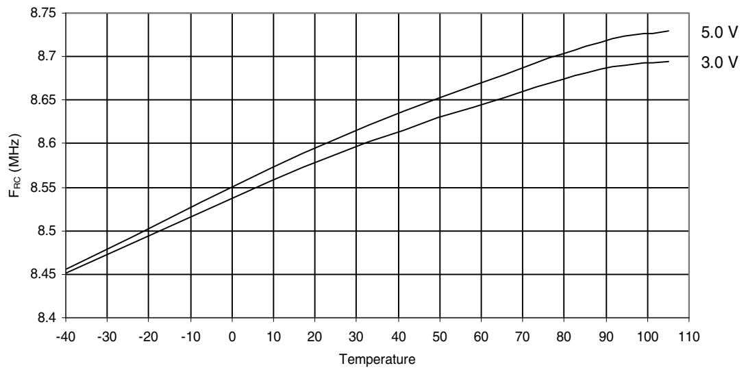
Figure 2-31. ATmega164P: Calibrated 8 MHz RC Oscillator vs. Temperature
