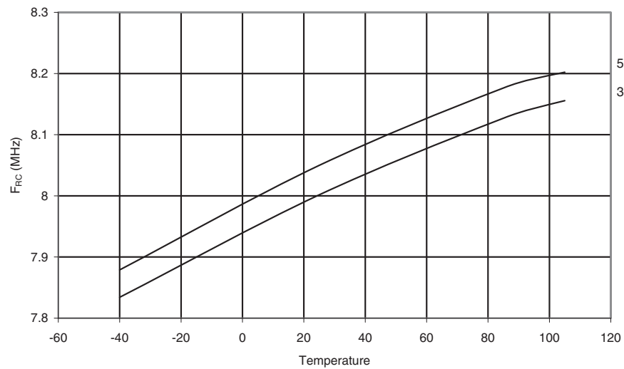
Figure 2-72. ATmega324P: Calibrated 8 MHz RC Oscillator vs. Temperature
