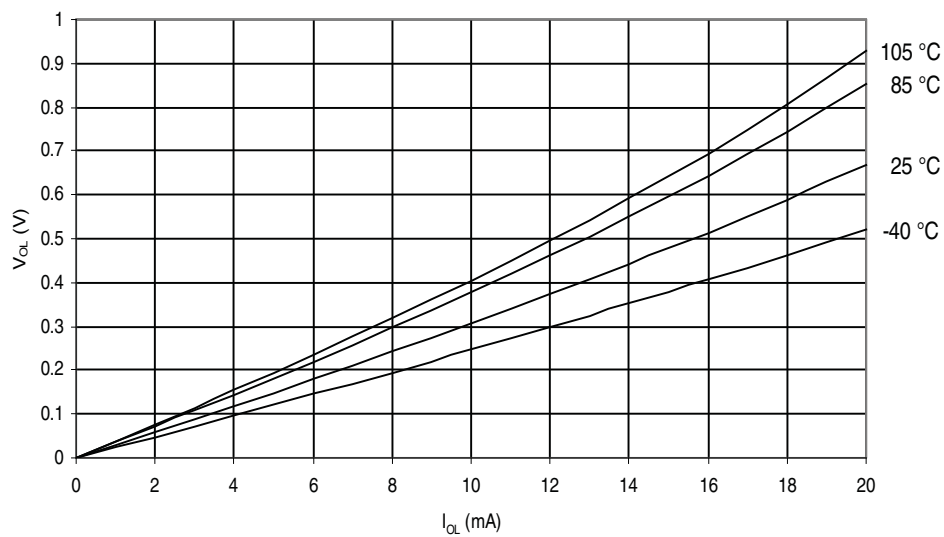
Figure 2-15. ATmega164P: I/O Pin Output Voltage vs. Sink Current ( V_{CC} = 3V )
