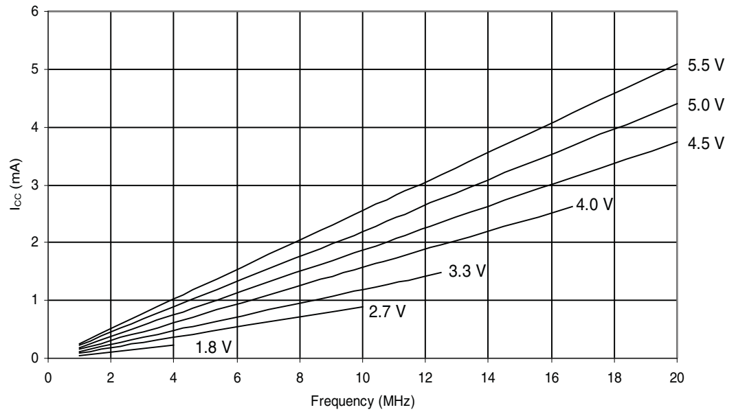
Figure 2-82. ATmega324P:Reset Supply Current vs Vcc 1-20MHz
