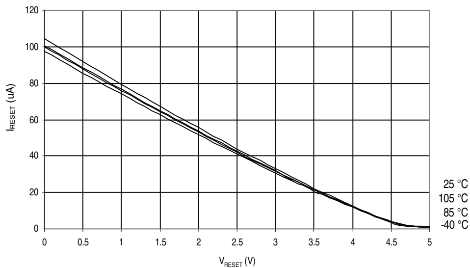
Figure 2-14. ATmega164P: Reset Pull-up Resistor Current vs. Reset Pin Voltage ( V_{CC} = 5V )
