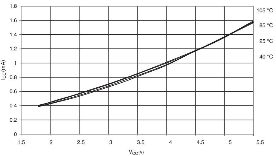
Figure 2-43. ATmega324P: Active Supply Current vs. V_{CC} (Internal RC Oscillator, 1 MHz)
