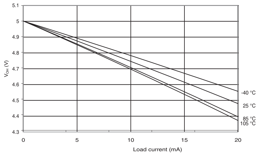
Figure 2-59. ATmega324P: I/O Pin Output Voltage vs. Source Current ( V_{CC} = 5V )
