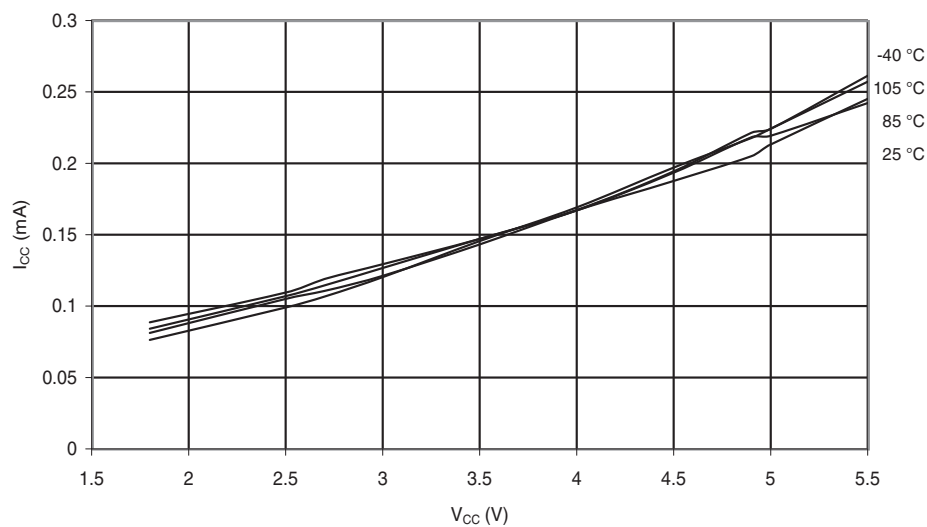
Figure 2-85. ATmega644P: Active Supply Current vs. V_{CC} (Internal RC Oscillator, 128 kHz).
