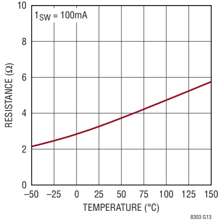
R_{DS(ON)}
