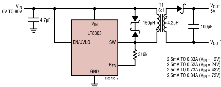
6V to 80V IN , 5V OUT Isolated Flyback Converter
