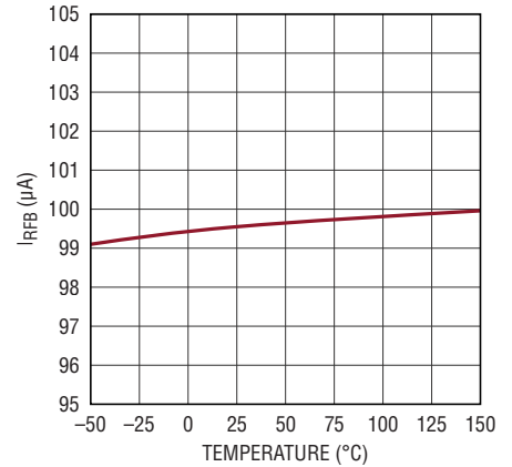
R_{FB} Regulation Current
