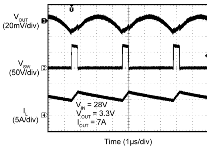
Switching Waveforms; I_{OUT} = 7A
