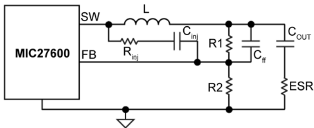
Figure 5c. Invisible Ripple at FB
