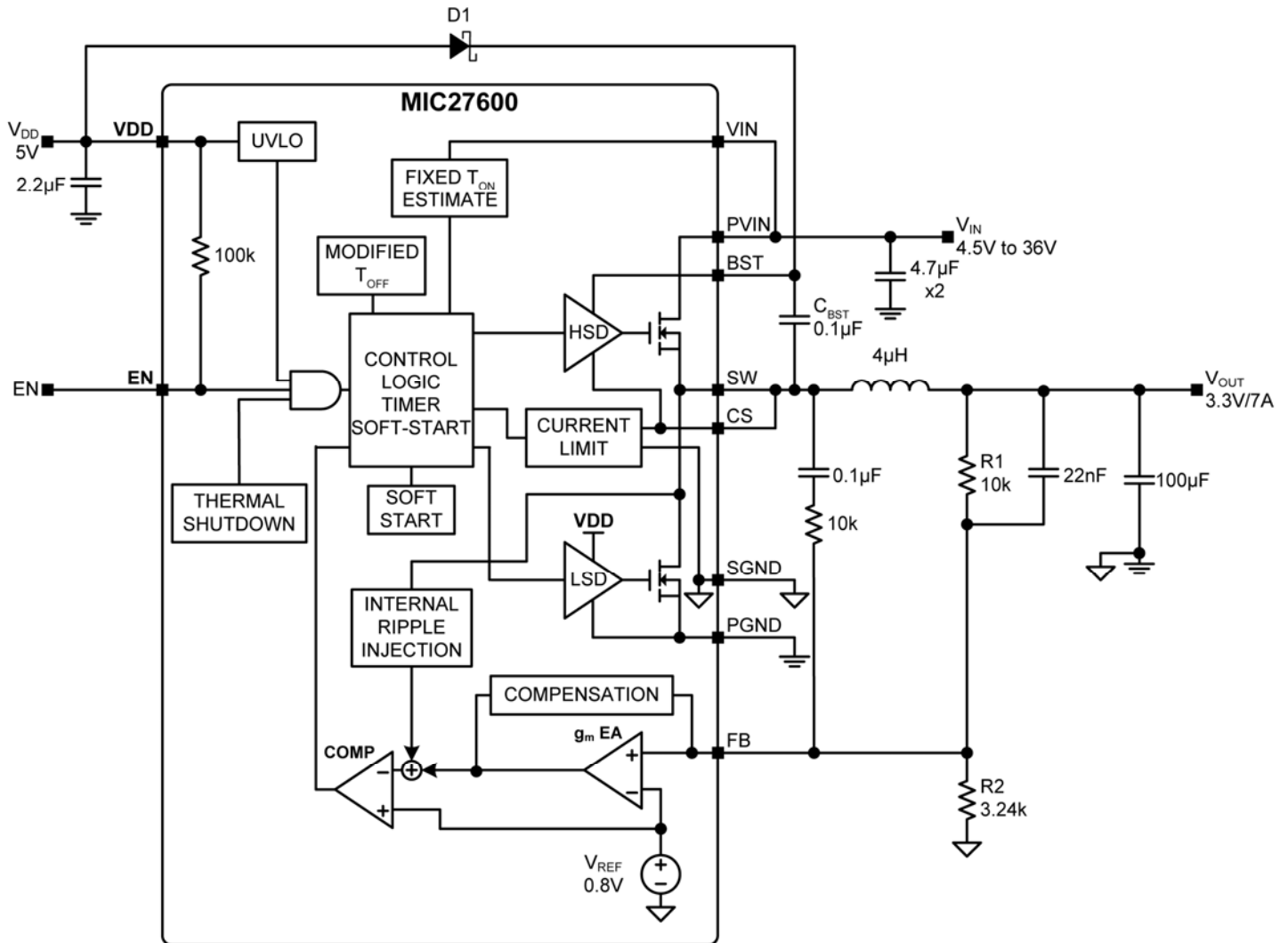
Figure 1. MIC27600 Block Diagram
