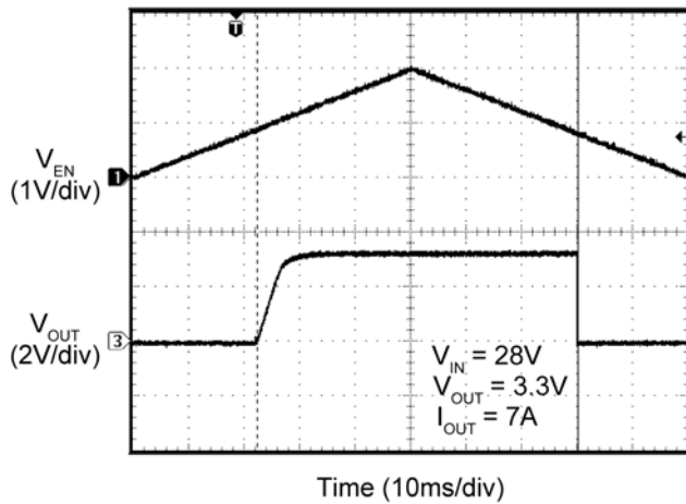
Enable Thresholds
