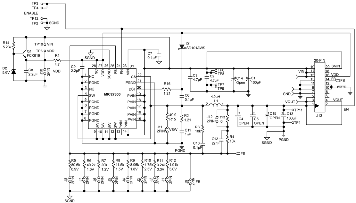
Figure 8. Schematic of MIC27600 Evaluation Board (J13, R13, R15 are for testing purposes)
