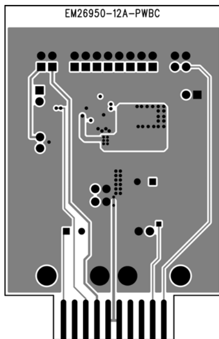
Figure 12. MIC27600 Evaluation Board Bottom Layer
