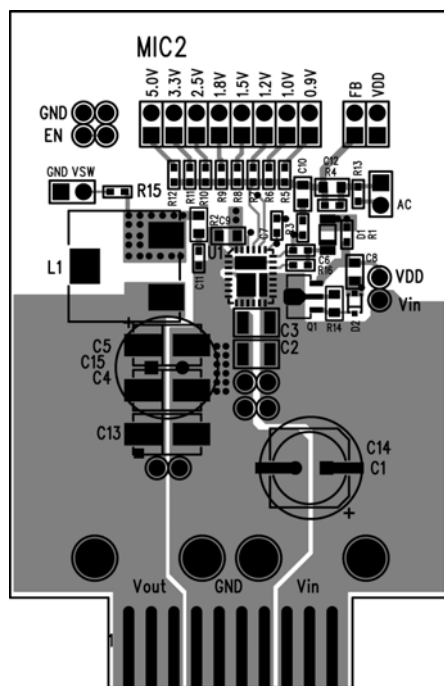
Figure 9. MIC27600 Evaluation Board Top Layer
