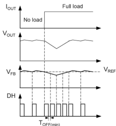
Figure 3. MIC27600 Load Transient Response
