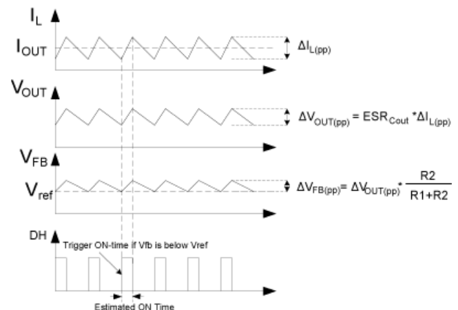
Figure 2. MIC27600 Control Loop Timing
