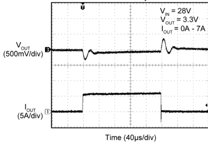
Transient Response
