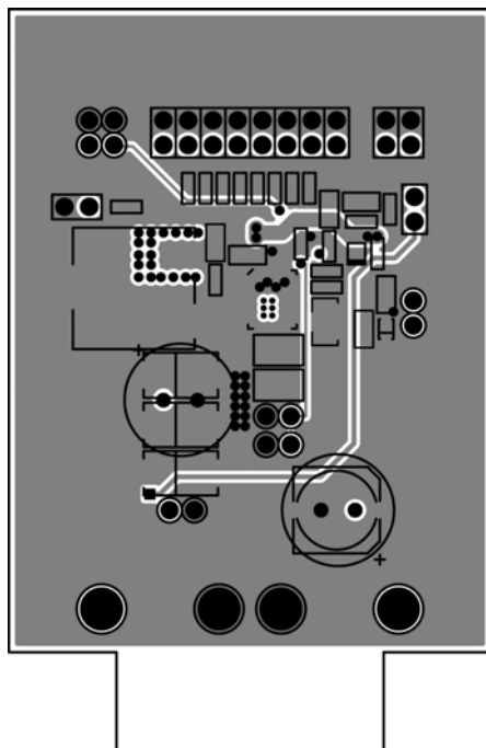
Figure 11. MIC27600 Evaluation Board Mid-Layer 2
