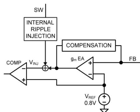
Figure 7. Internal Ripple Injection
