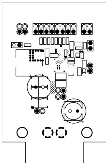
Figure 10. MIC27600 Evaluation Board Mid-Layer 1 (Ground Plane)
