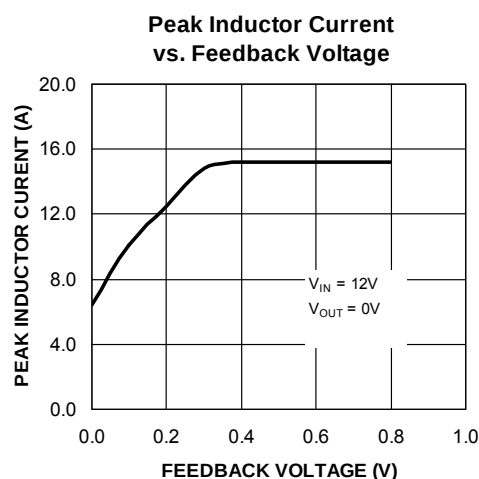
Figure 4. MIC27600 Current Limit Foldback Characteristic
