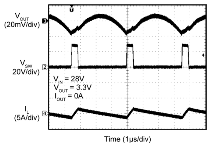
Switching Waveforms; I_{OUT} = 0A
