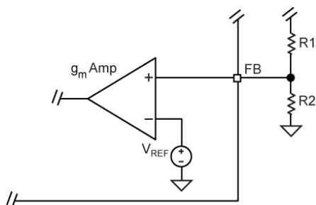
Figure 6. Voltage-Divider Configuration
