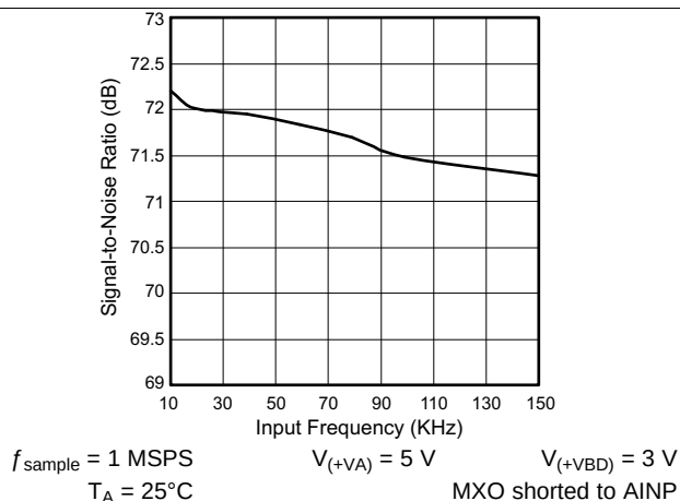
Figure 25. Signal-to-Noise Ratio vs Input Frequency
