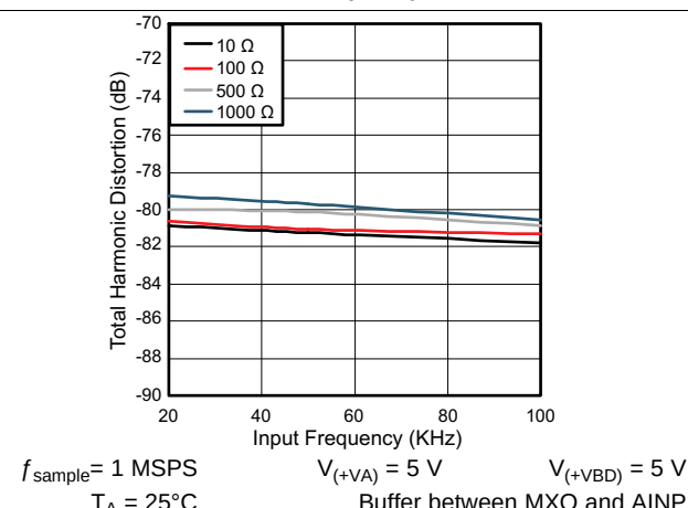
Figure 30. Total Harmonic Distortion vs Input Frequency (Across Different Source Resistance Values)
