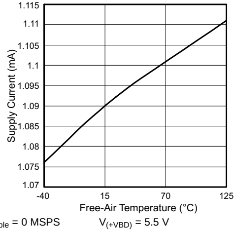
Figure 4. Idle Supply Current ( I_{(+VA)} ) vs Free-Air Temperature
