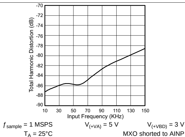
Figure 27. Total Harmonic Distortion vs Input Frequency
