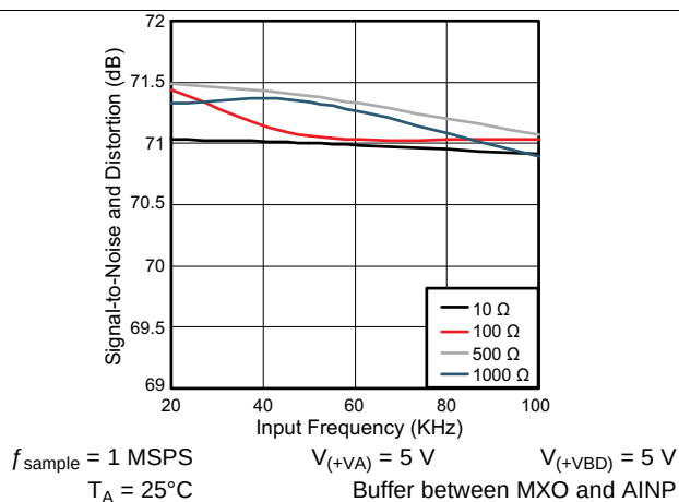
Figure 29. Signal-to-Noise With Distortion vs Input Frequency (Across Different Source Resistance Values)
