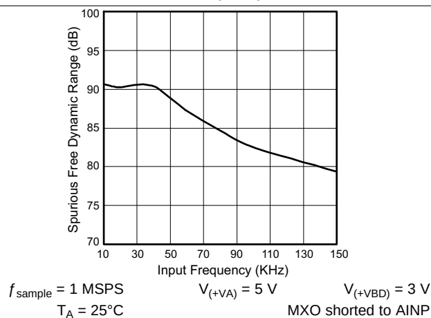
Figure 28. Spurious-Free Dynamic Range vs Input Frequency
