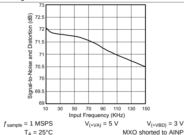
Figure 26. Signal-to-Noise With Distortion vs Input Frequency
