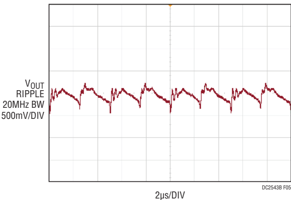
Figure 5. Output Voltage Ripple at V_{IN} = 48V , V_{OUT} = 24V , I_{OUT} = 10A , f_{SW} = 200kHz
