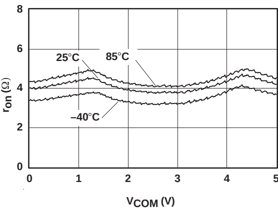
Figure 2. r_{on} vs V_{COM} ( V_+ = 5V )
