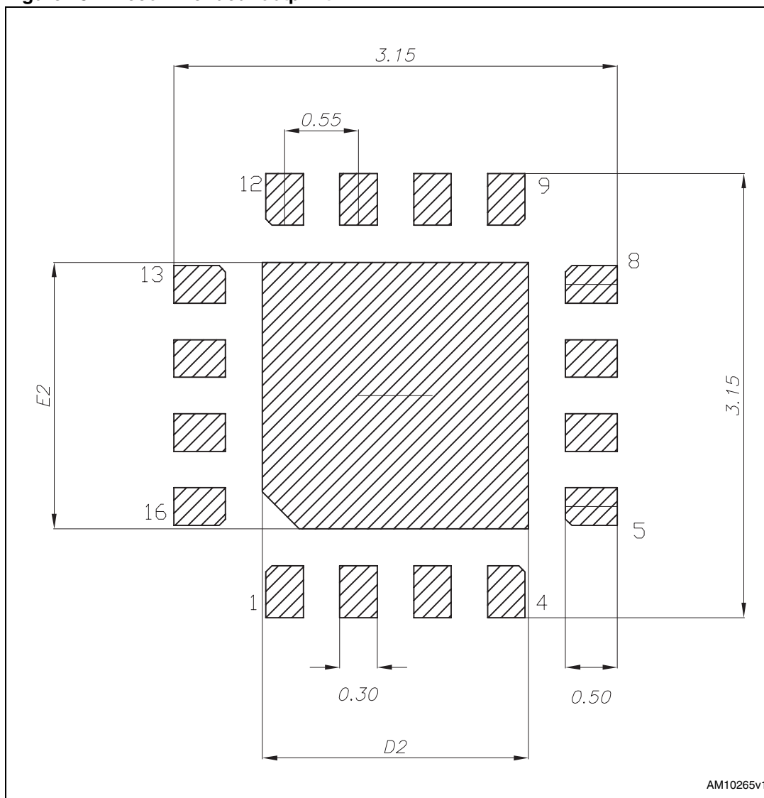
Figure 15. Recommended footprint
