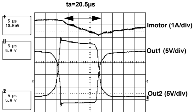
Figure 18. Switch off Time
