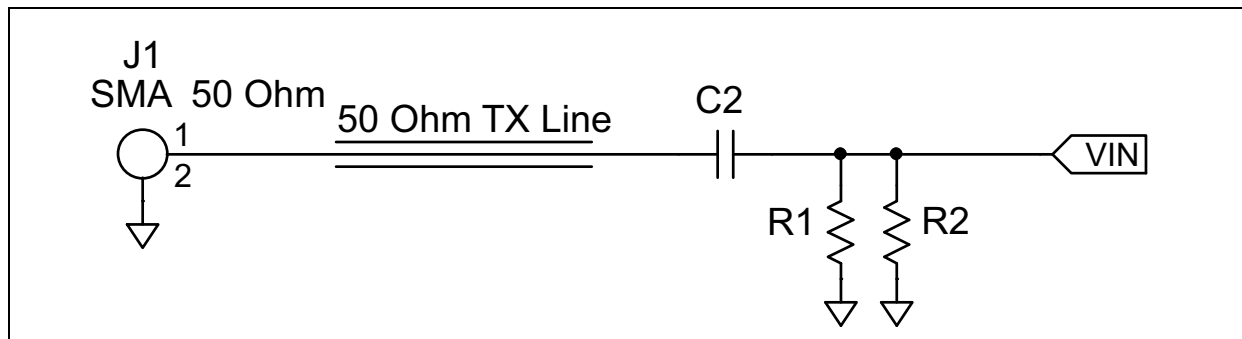
FIGURE 2-4: Input Stage Block.
