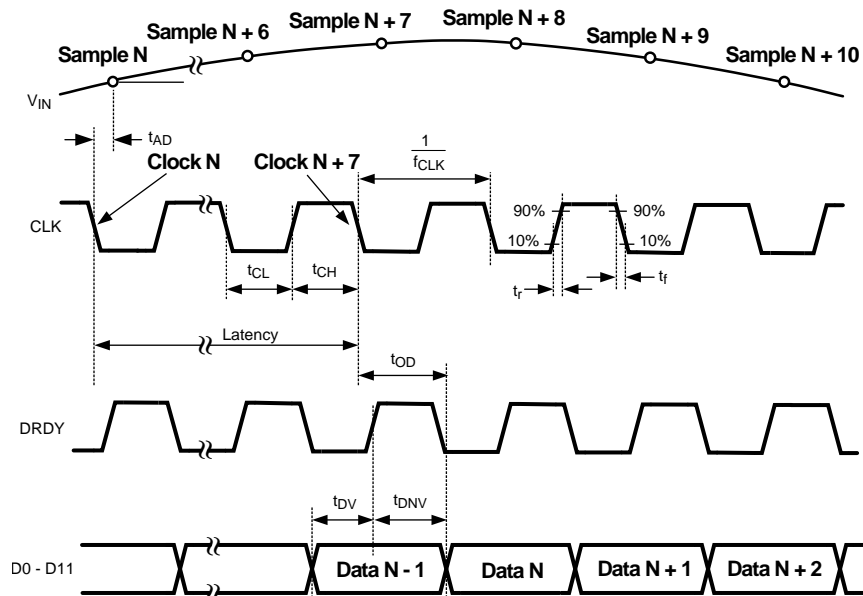
Figure 1. Output Timing
