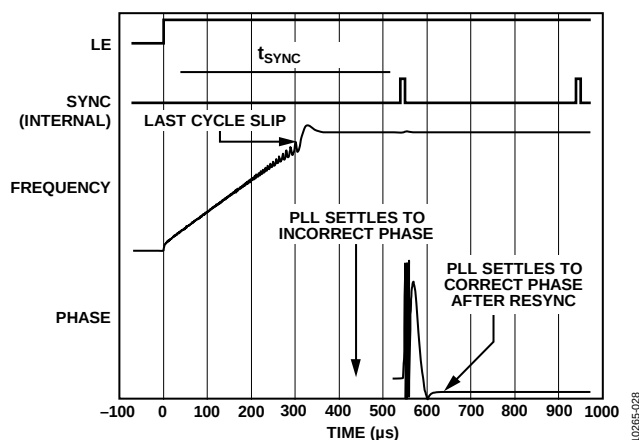
Figure 28. Phase Resync Example
