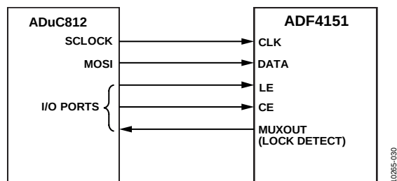
Figure 30. ADuC812 to ADF4151 Interface
