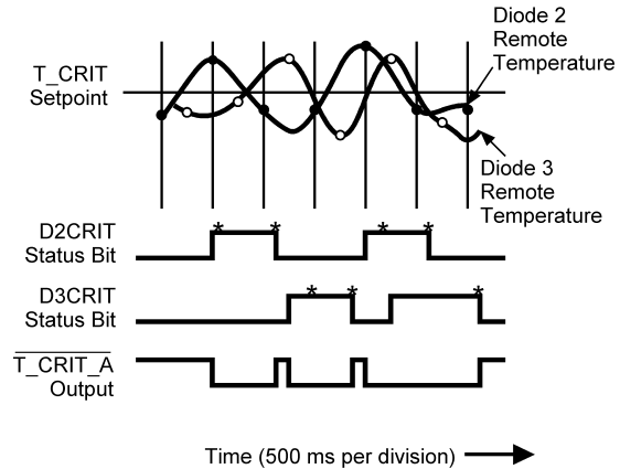
FIGURE 6. \overline{\text{T\_CRIT\_A}} Temperature Response Diagram with remote diode 1 and local temperature masked.
