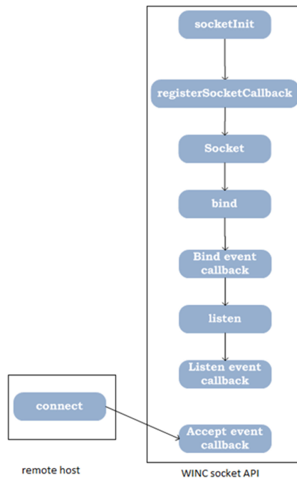
Figure 6-2. TCP Server API Call Sequence
