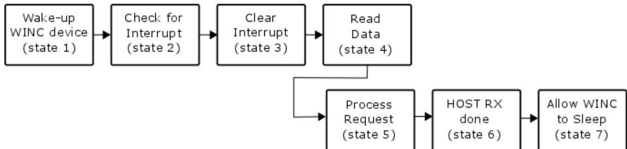
Figure 13-4. HIF Frame Receive from WINC to Host
