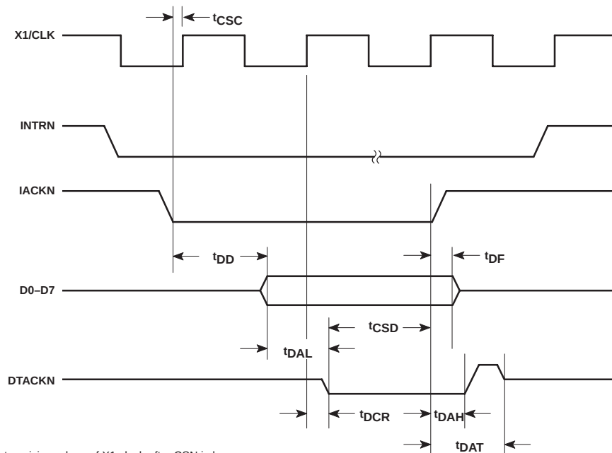
Figure 6. Interrupt Cycle Timing
