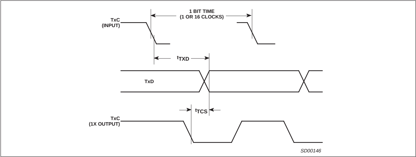
Figure 10. Transit Timing
