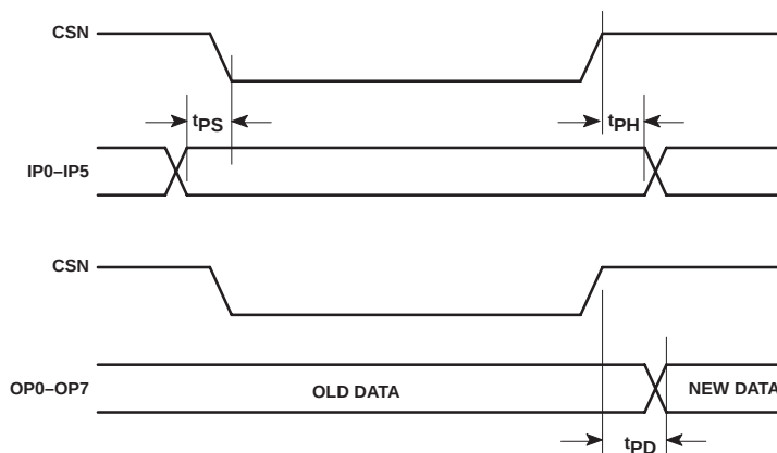
Figure 7. Port Timing
