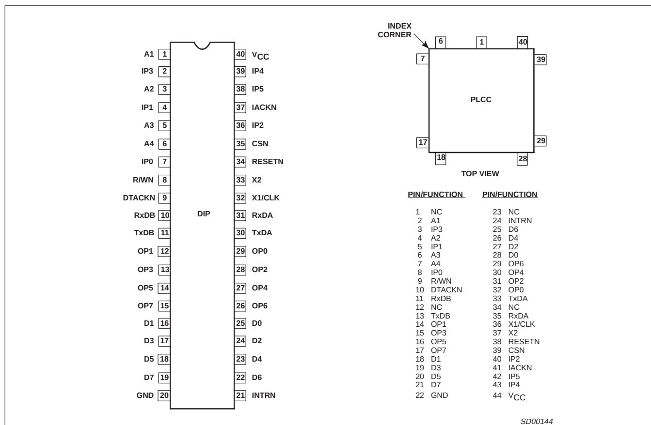
Figure 1. Pin Configurations
