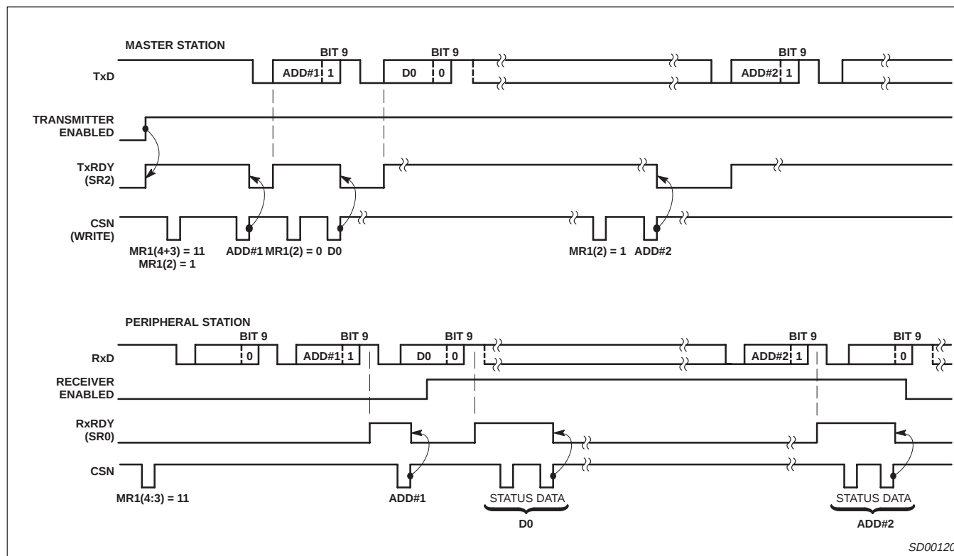
Figure 14. Wake-Up Mode
