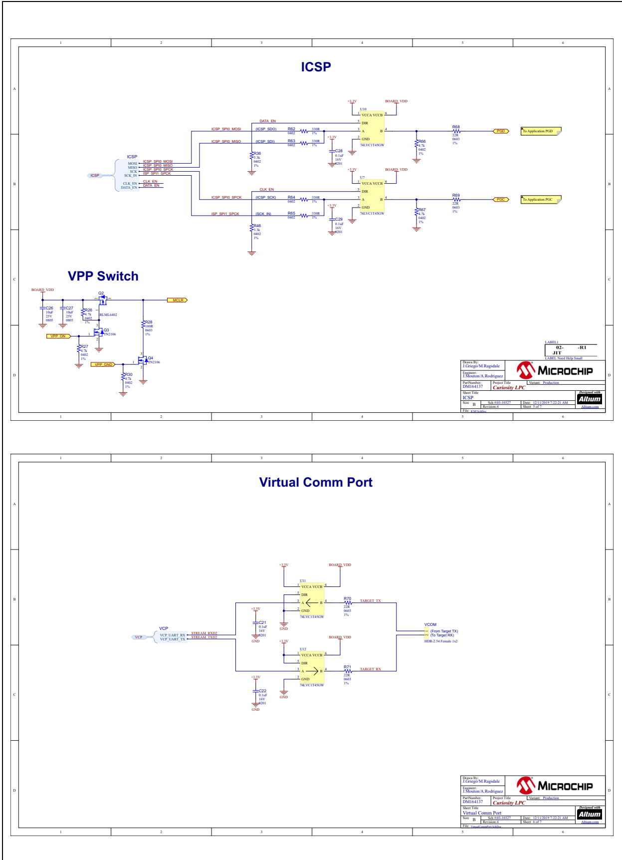
FIGURE A-4: CURIOSITY LPC DEVELOPMENT BOARD SCHEMATIC REV 4 (3 OF 4)
