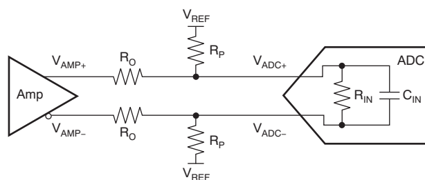
Figure 38. Resistor Network to DC Level-Shift Common-Mode Voltage
