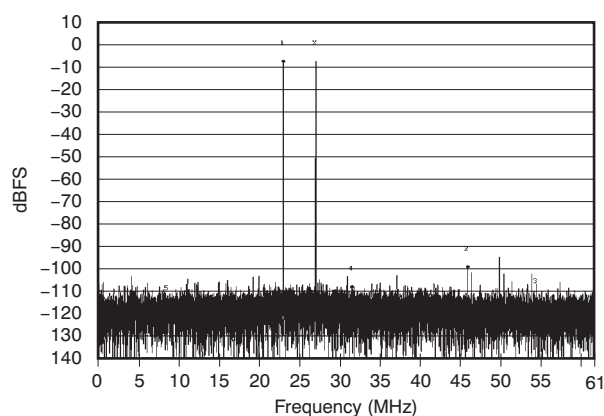
Figure 40. FFT Plot of THS770006 + 30MHz BPF + 16-Bit ADC with Two-Tone Input at 96MHz and 100MHz
