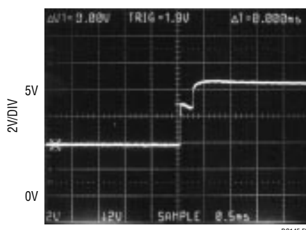
Figure 2. V GS of N-Channel MOSFET Switch Being Turned On
