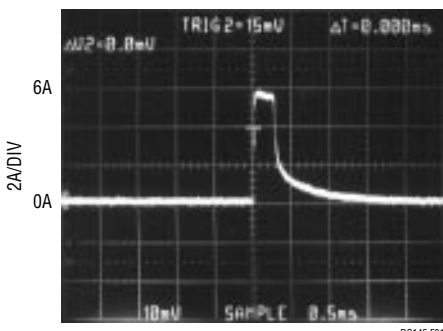
Figure 1. Inrush Current from a 24V Battery into a 100μF Capacitor
