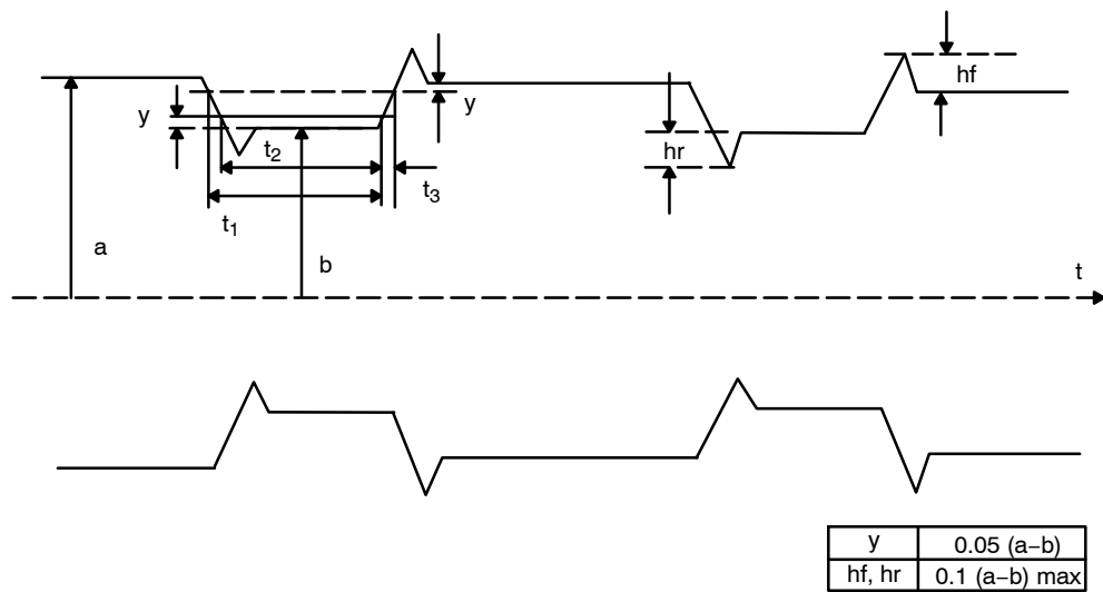
Figure 3. 10% Modulation Waveform
