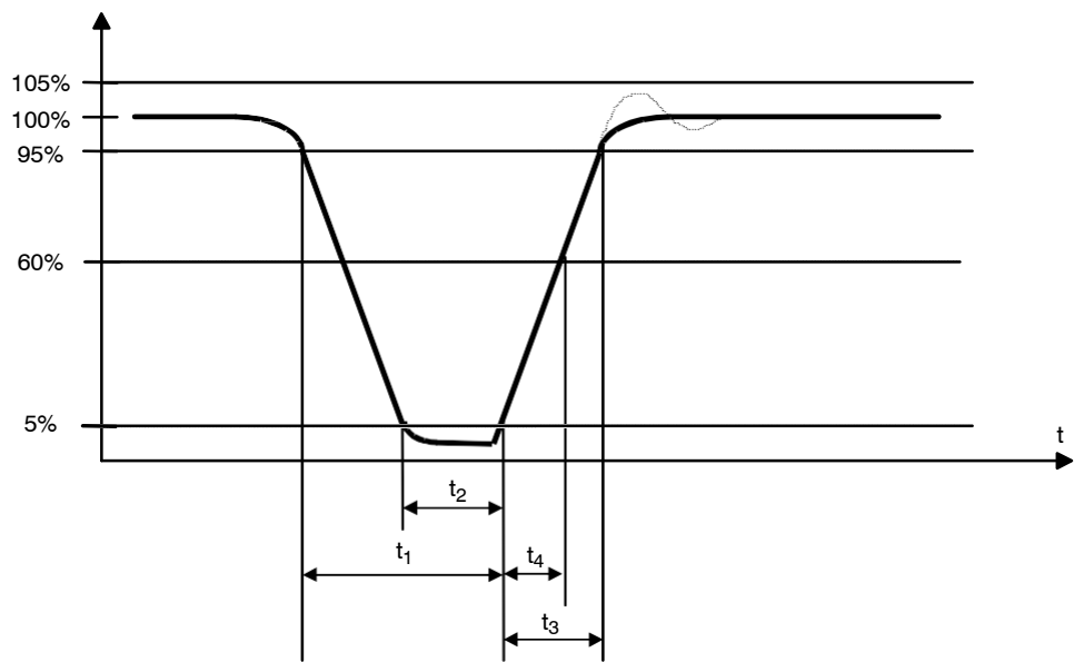
Figure 2. 100% Modulation Waveform
