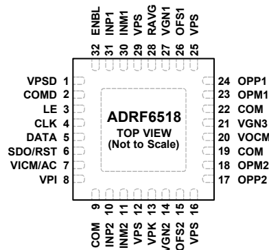
Figure 4. Pin Configuration
