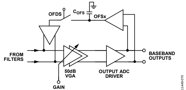
Figure 71. Offset Compensation Loop Operates Around the VGA and Output Buffer
