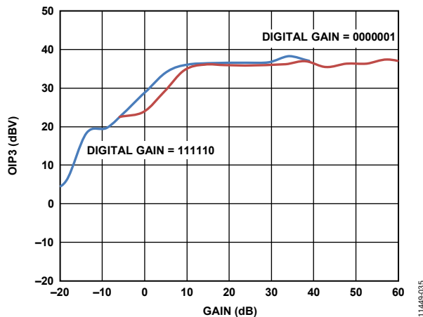
Figure 37. In-Band OIP3 vs. Gain over Digital Gain; 1.5 V p-p Composite Output Target, 30 MHz and 31 MHz Tones
