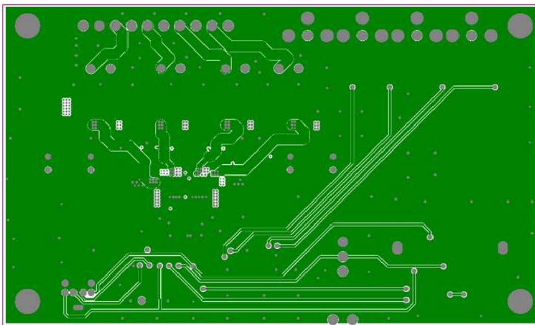
Figure 14. TAS5414CDKD Mid Layer Level 1
