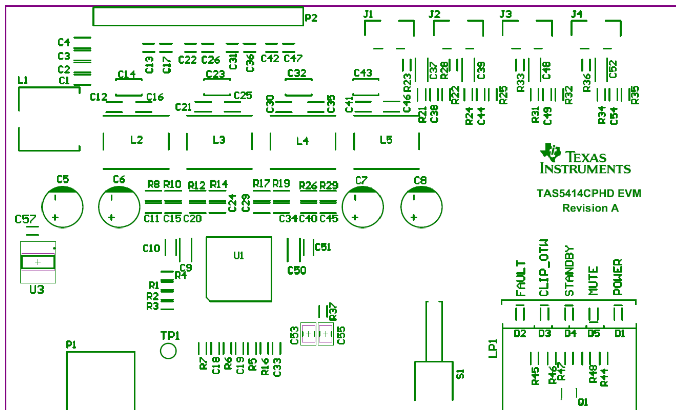
Figure 11. TAS5414CPHD Top Silkscreen Overlay
