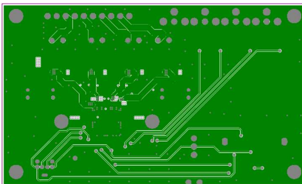
Figure 8. TAS5414CPHD Mid Layer Level 1
