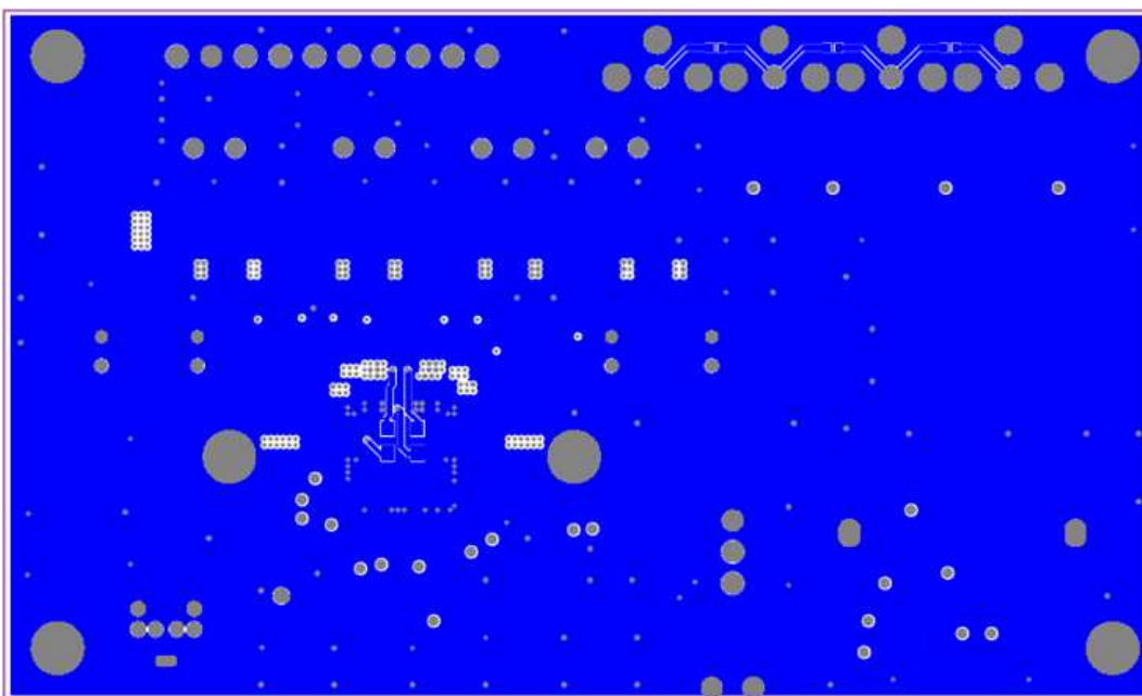
Figure 10. TAS5414CPHD Bottom Layer
