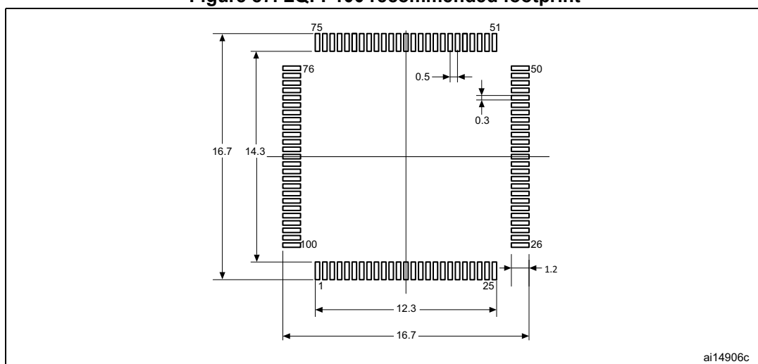
Figure 87. LQFP100 recommended footprint
