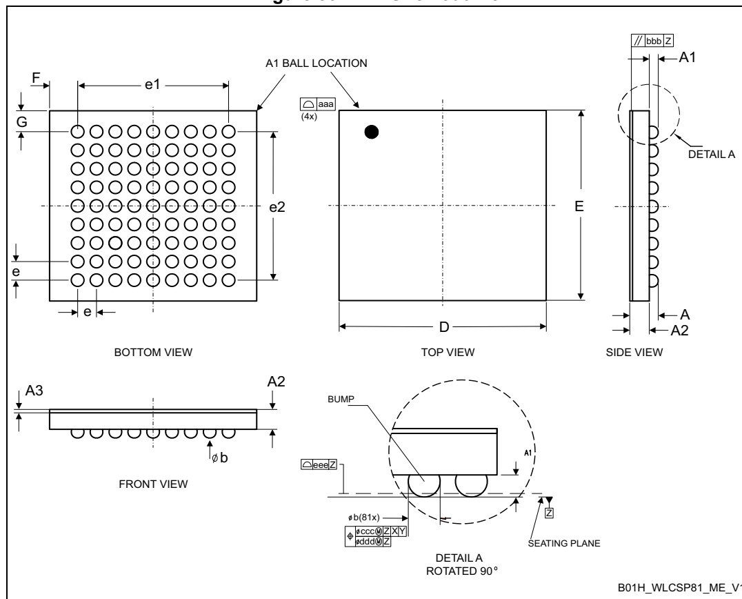
Figure 83. WLCSP81 outline
