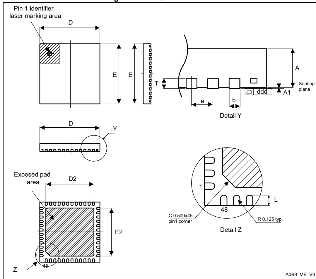
Figure 77. UFQFPN48 outline
