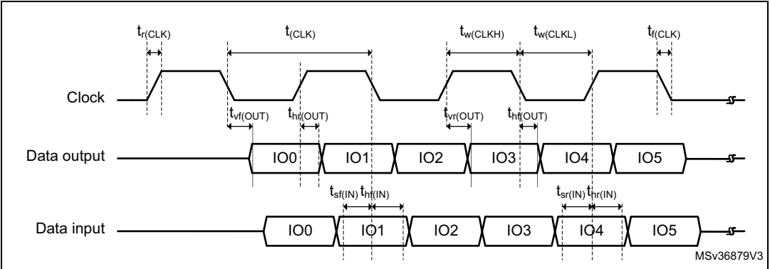
Figure 66. OCTOSPI timing diagram - DDR mode
