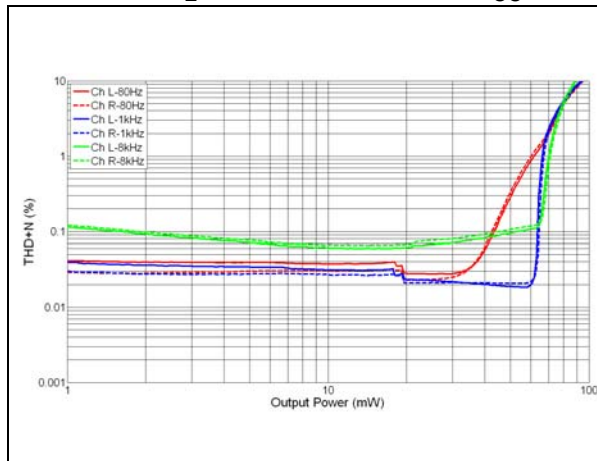
Figure 16. THD+N vs. output power - R_L = 16 \Omega , out-of-phase, V_{CC} = 4.8 V
