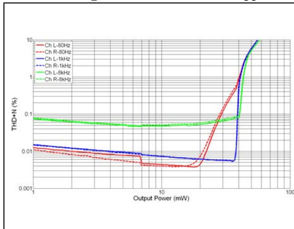
Figure 20. THD+N vs. output power - R_L = 32 \Omega , out-of-phase, V_{CC} = 3.6 V
