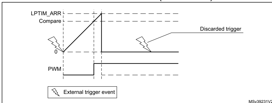
Figure 198. LPTIM output waveform, Single counting mode configuration and Set-once mode activated (WAVE bit is set)
