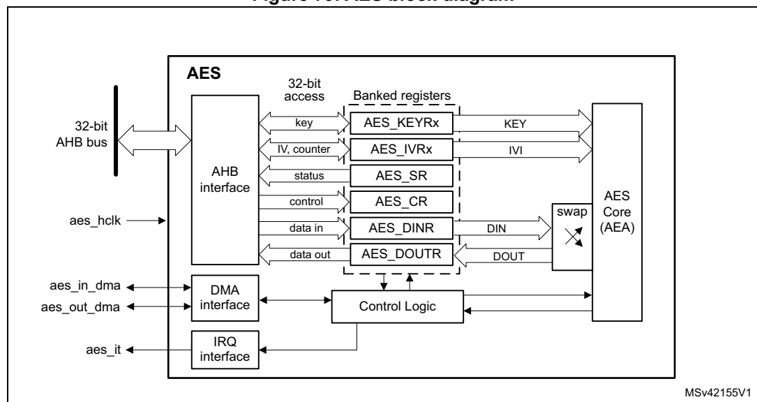
Figure 79. AES block diagram
