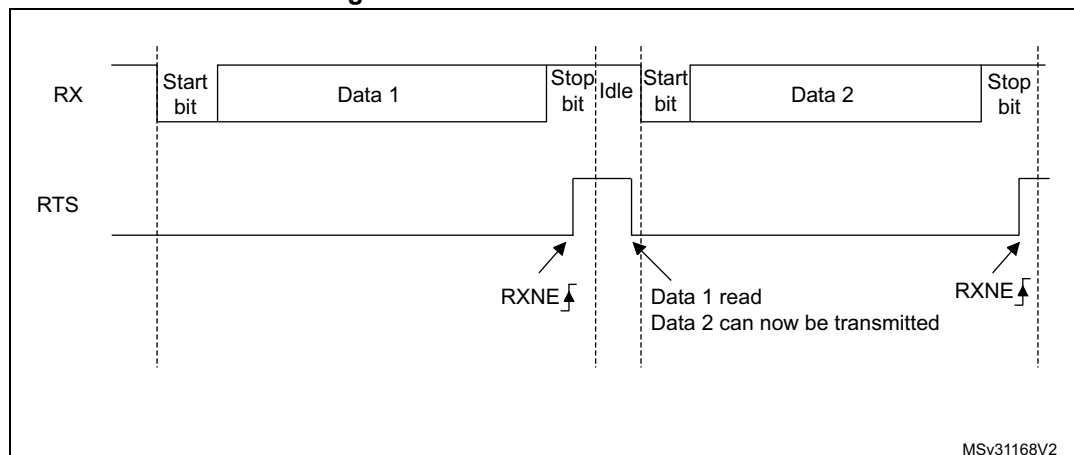
Figure 260. RS232 RTS flow control
