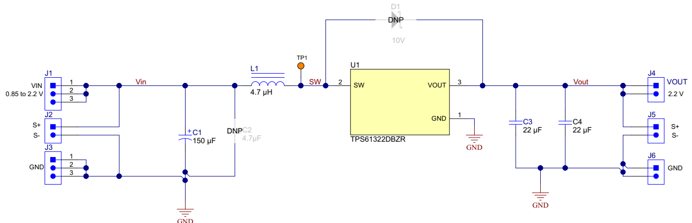
Figure 1. TPS61322EVM-001 Schematic
