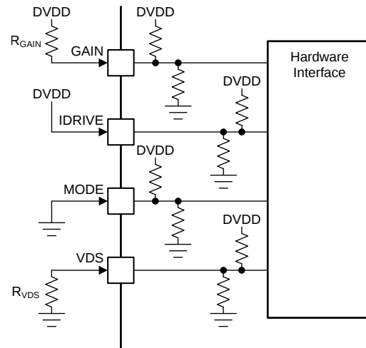
Figure 24. Hardware Interface
