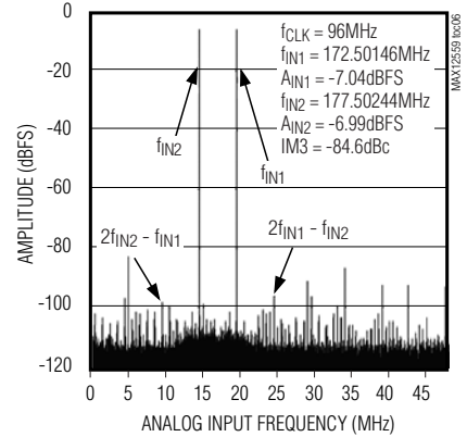
TWO-TONE IMD PLOT (65,536-POINT DATA RECORD)
