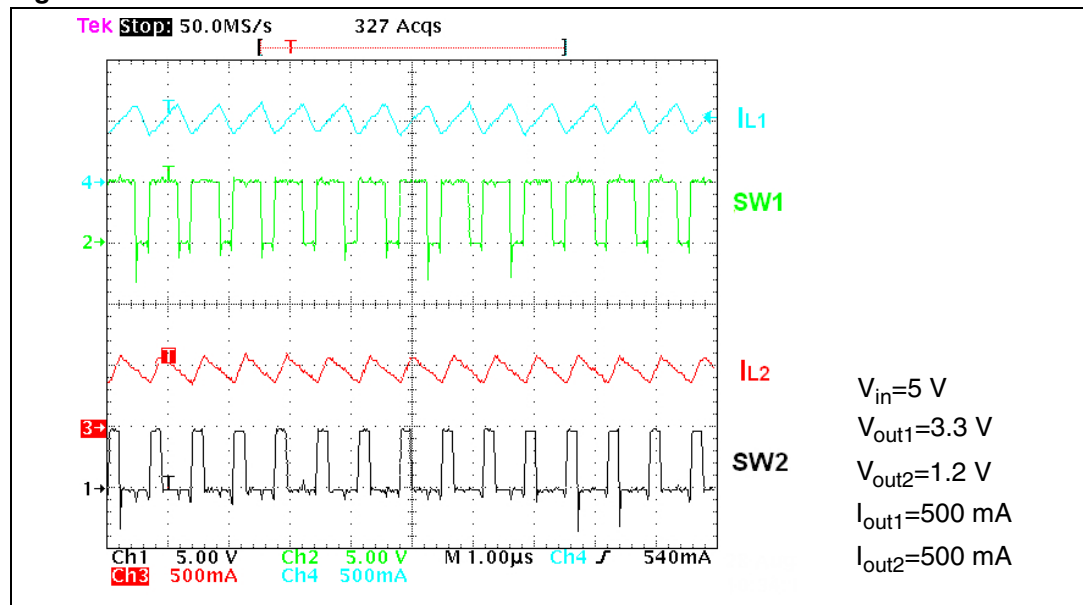
Figure 4. Inductor current in PWM
