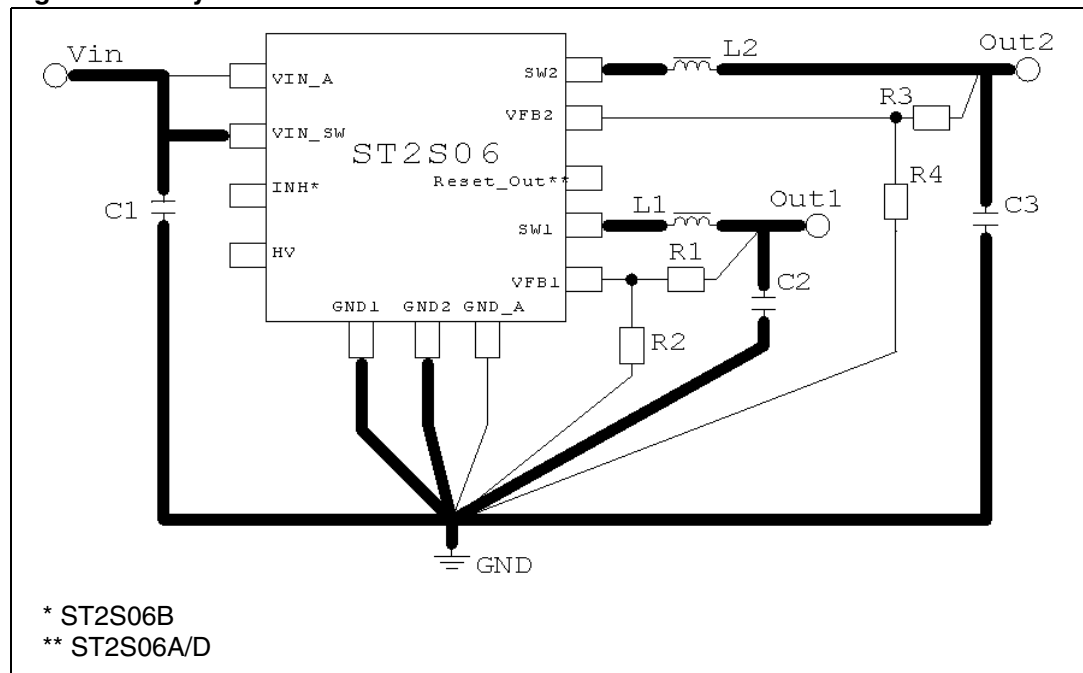
Figure 16. Layout considerations
