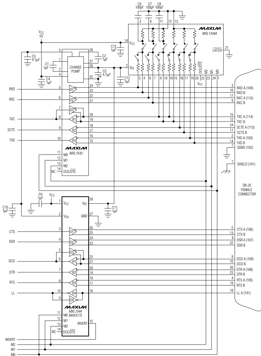
Figure 17. Controller-Selectable DCE Port with DB-25 Connector
