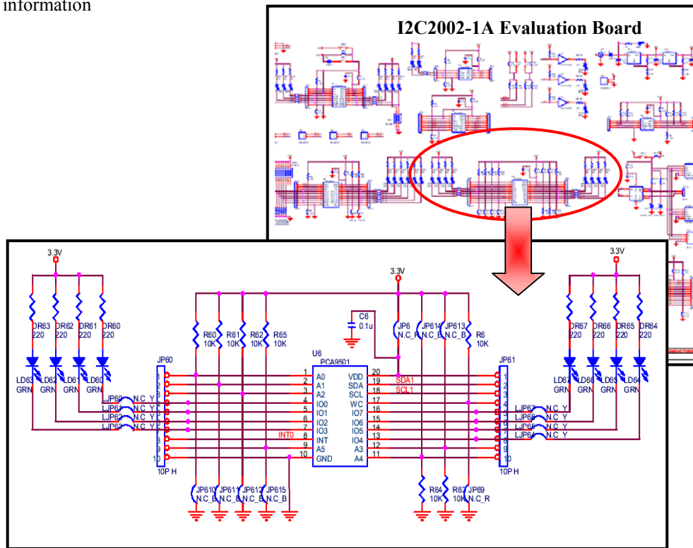
Figure 7. PCA9501 Schematic
