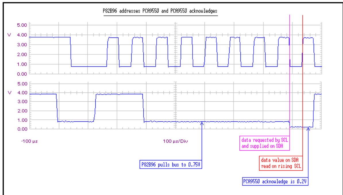
Figure 28. P82B96 waveforms
