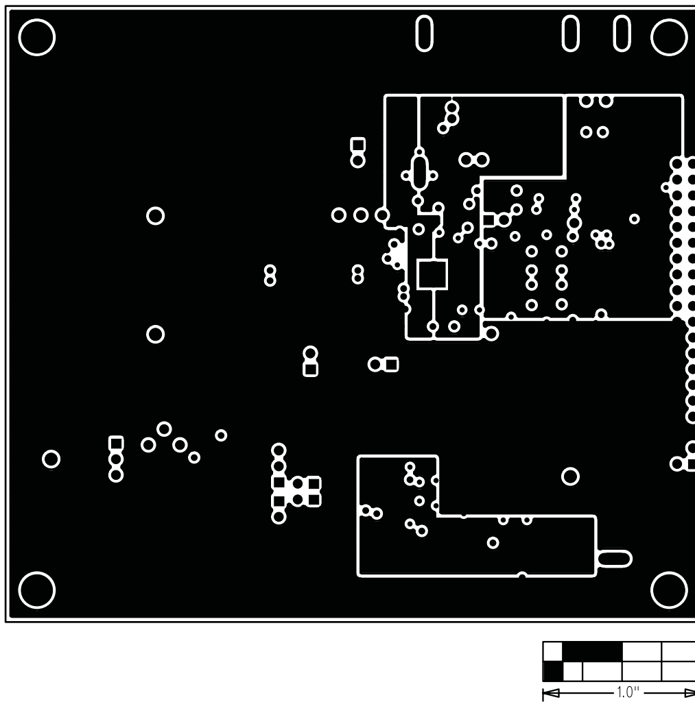
Figure 5. MAX12553/MAX12554/MAX12555 EV Kits PCB Layout—Power Planes
