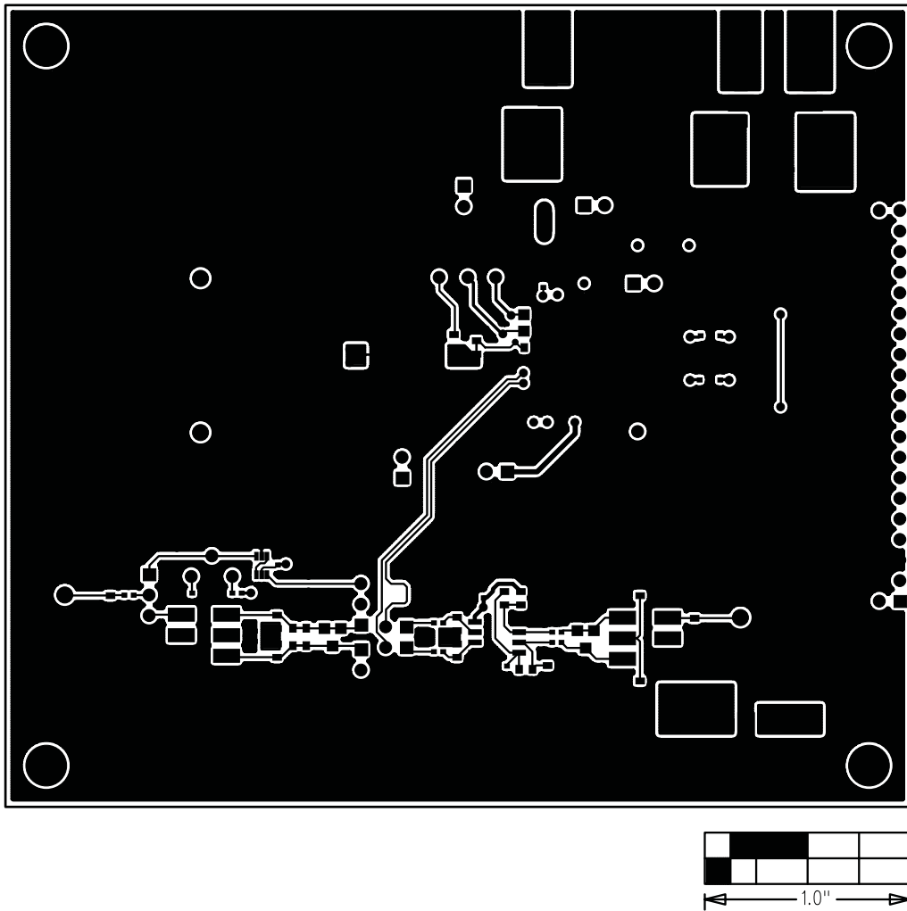
Figure 6. MAX12553/MAX12554/MAX12555 EV Kits PCB Layout—Solder Side
