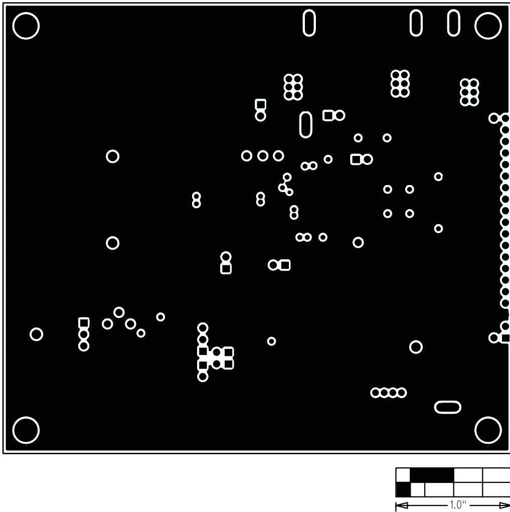
Figure 4. MAX12553/MAX12554/MAX12555 EV Kits PCB Layout—Ground Planes
