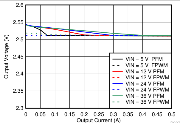
Figure 67. Line and Load Regulation
