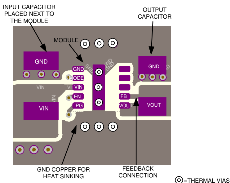
Figure 82. Layout Example With Fixed Output Version
