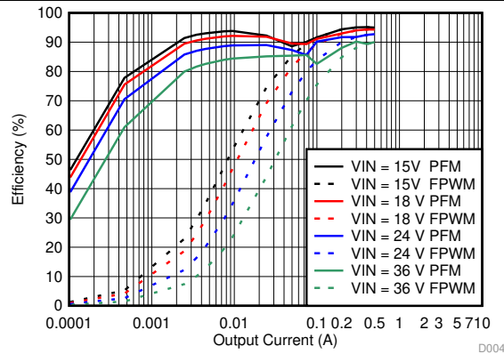
Figure 51. Efficiency
