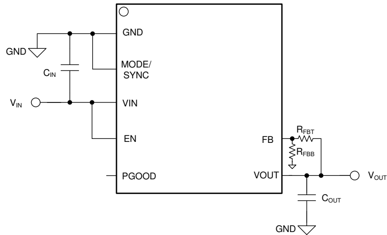
Figure 35. Adjustable 1.2-V to 15-V Output Typical Application Circuit
