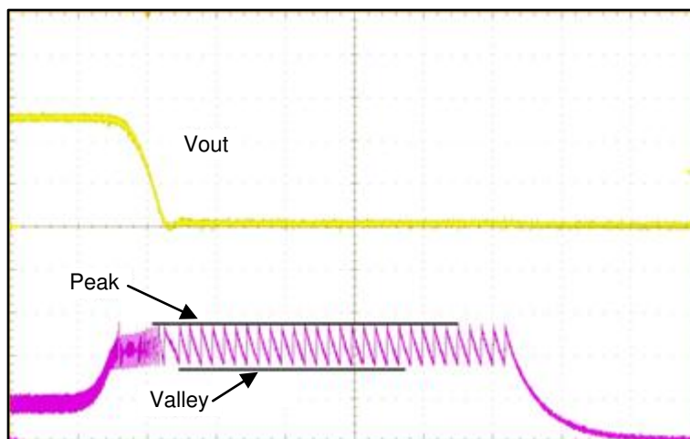
Figure 32. Current Limit Operation During Output Short Circuit
