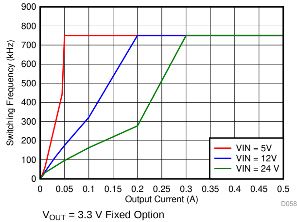
Figure 25. Auto PFM Mode Switching Frequency vs Output Current
