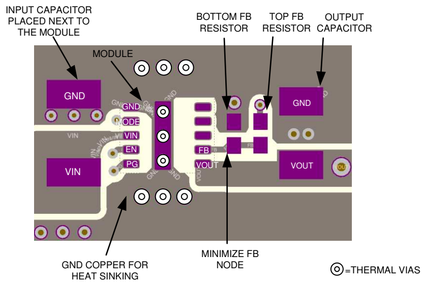
Figure 83. Layout Example With Adjustable Output Version
