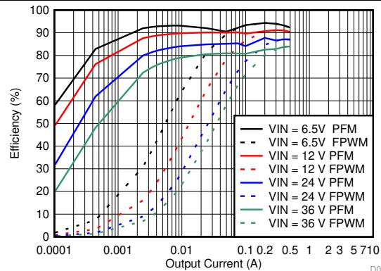
Figure 75. Efficiency for V_{OUT} = 5\text{ V}
