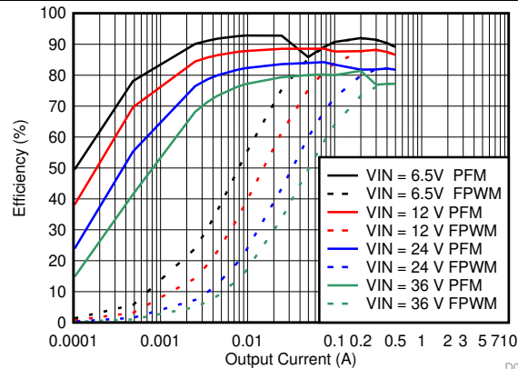
Figure 45. Efficiency
