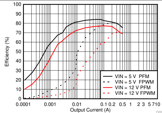
Figure 70. Efficiency for V_{OUT} = 1.2\text{ V}
