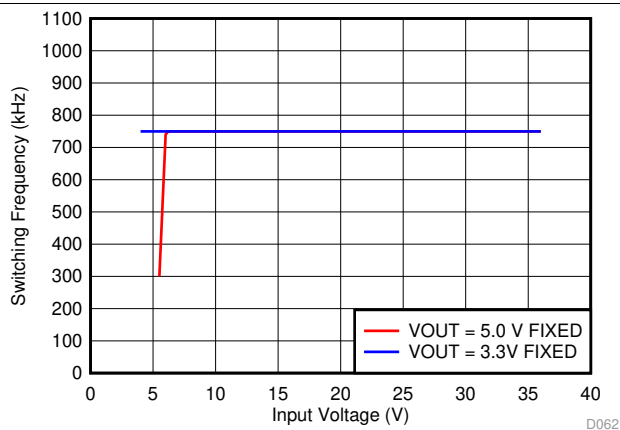
Figure 31. Switching Frequency vs Input Voltage for Fixed Output Options at Full Load
