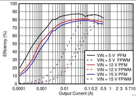
Figure 69. Efficiency for V_{OUT} = 1.8\text{ V}
