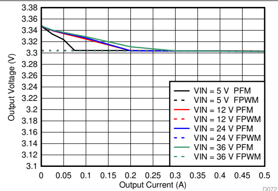
Figure 78. Line and Load Regulation for V_{OUT} = 3.3\text{ V}
