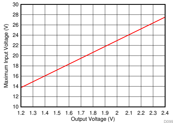
Figure 36. Maximum Input Voltage for V_{OUT} < 2.5\text{ V}
