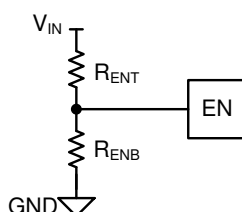
Figure 38. Enable Divider to Set External UVLO Threshold
