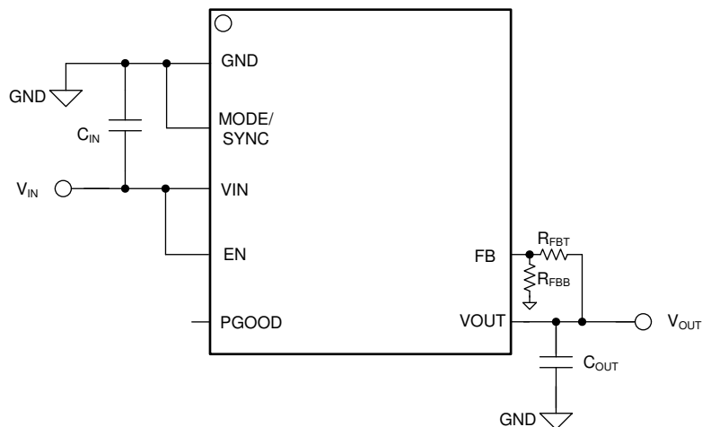
Figure 37. Adjustable 1.2-V to 15-V Output Typical Application Circuit
