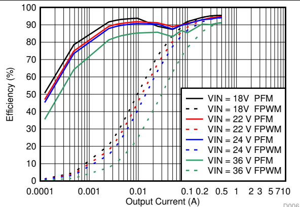
Figure 57. Efficiency
