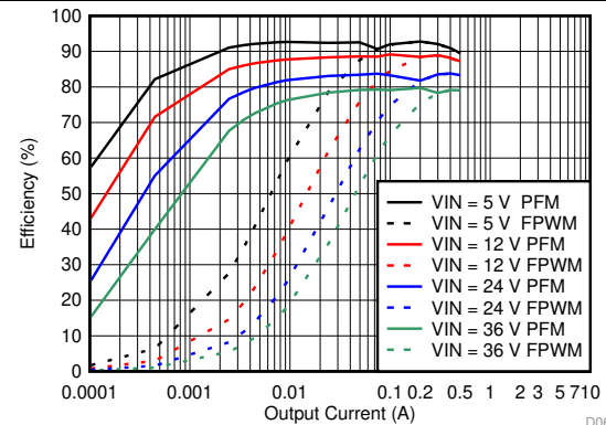
Figure 76. Efficiency for V_{OUT} = 3.3\text{ V}
