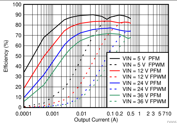
Figure 63. Efficiency
