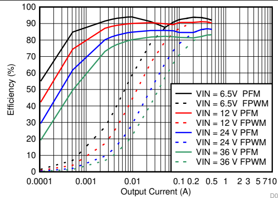
Figure 39. Efficiency
