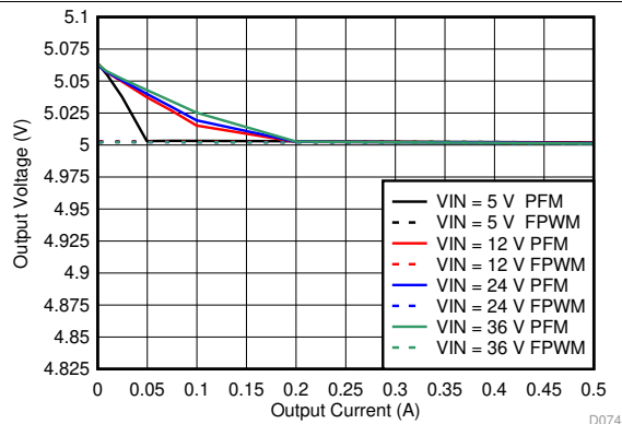
Figure 77. Line and Load Regulation for V_{OUT} = 5\text{ V}
