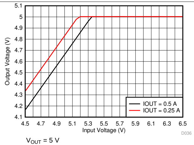
Figure 4. Dropout Voltage
