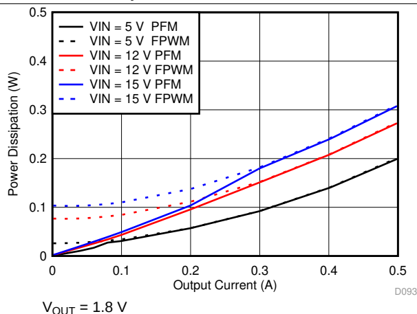
Figure 14. Power Dissipation
