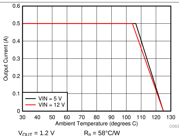
Figure 16. Ambient Temperature vs Output Current
