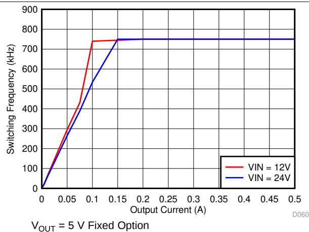
Figure 27. Auto PFM Mode Switching Frequency vs Output Current
