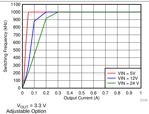
Figure 24. Auto PFM Mode Switching Frequency vs Output Current
