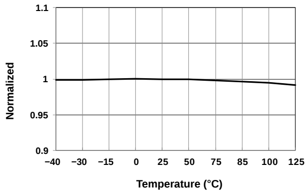
Figure 19. RLR Pin Source Current ( I_{PLR} ) vs. Temperature
