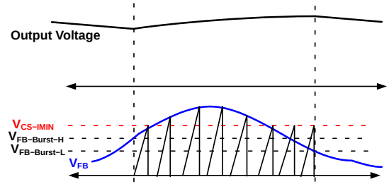
Figure 21. Burst-Mode Operation
