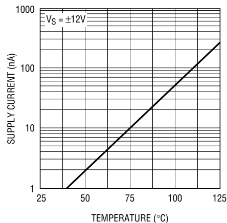
Off Supply Current vs Temperature
