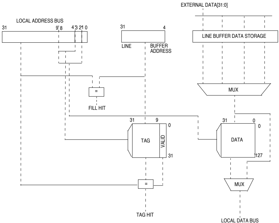
Figure 4-1. Instruction Cache Block Diagram
