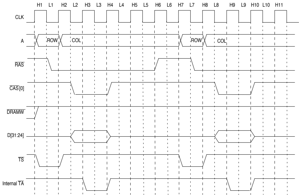
Figure 10-10. Byte Read Transfer Followed by a Page-Miss Byte Read Transfer in Fast Page Mode with 8-Bit DRAM
