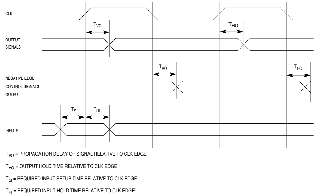
Figure 6-1. Signal Relationships to CLK
