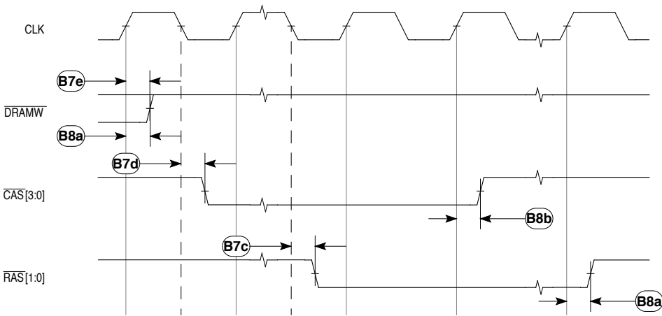
DRAM Refresh Cycle Timing
