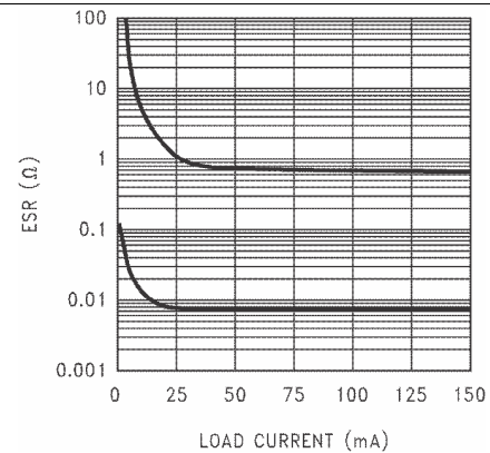
Figure 18. 2.2-μF Stable ESR Range for Output Voltage ≤ 2.3 V
