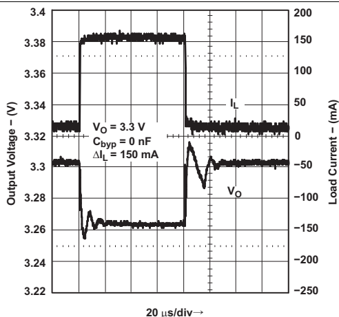
Figure 23. Load Transient Response
