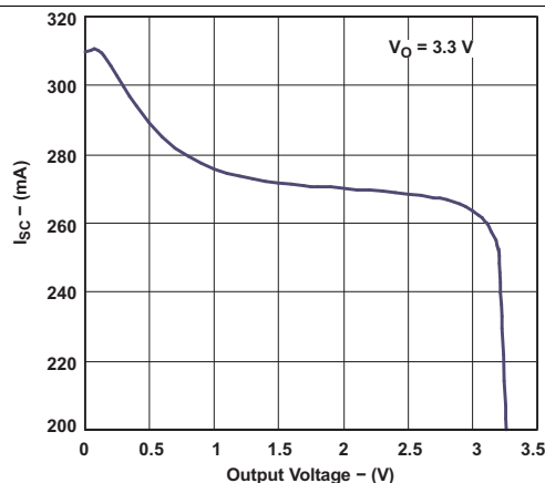
Figure 6. Short-circuit Current vs Output Voltage
