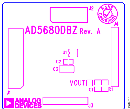
Figure 13. EVAL-AD5680DBZ Daughter Board Component Placement
