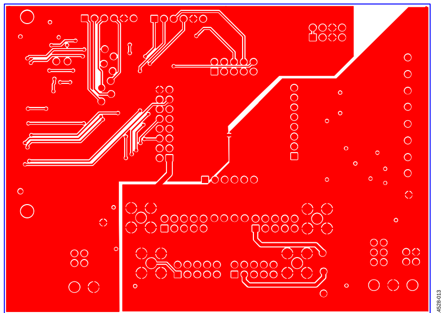
Figure 11. EVAL-MBnanoDAC-SDZ Motherboard Bottom Side Routing
