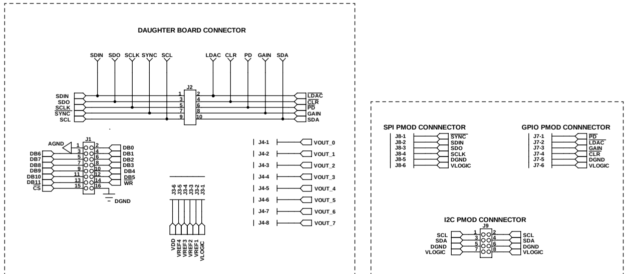
Figure 7. EVAL-MBnanoDAC-SDZ Motherboard Connectors to Daughter Board and Serial Interface
