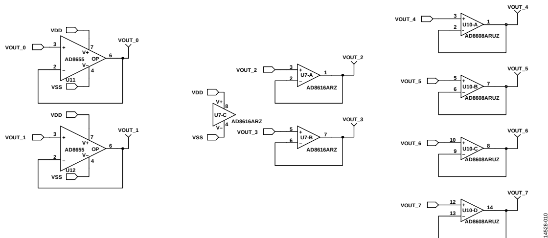
Figure 8. EVAL-MBnanoDAC-SDZ Motherboard Output Amplifier Circuit
