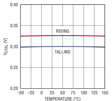
CTRL Latch-Off Threshold
