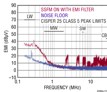
Figure 10. Peak Conducted EMI
