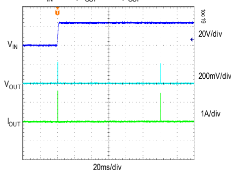
OUTPUT SHORT DURING STARTUP
