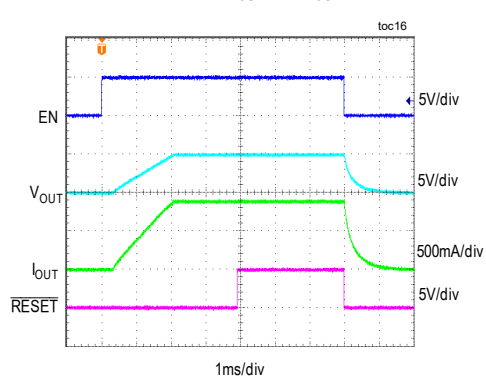
STARTUP AND SHUTDOWN THROUGH ENABLE
