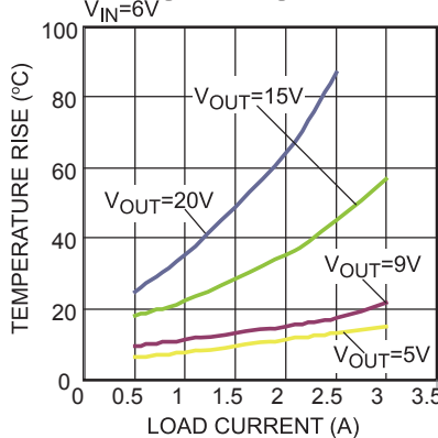
MP3428A Case Temperature Rising For Figure 11
